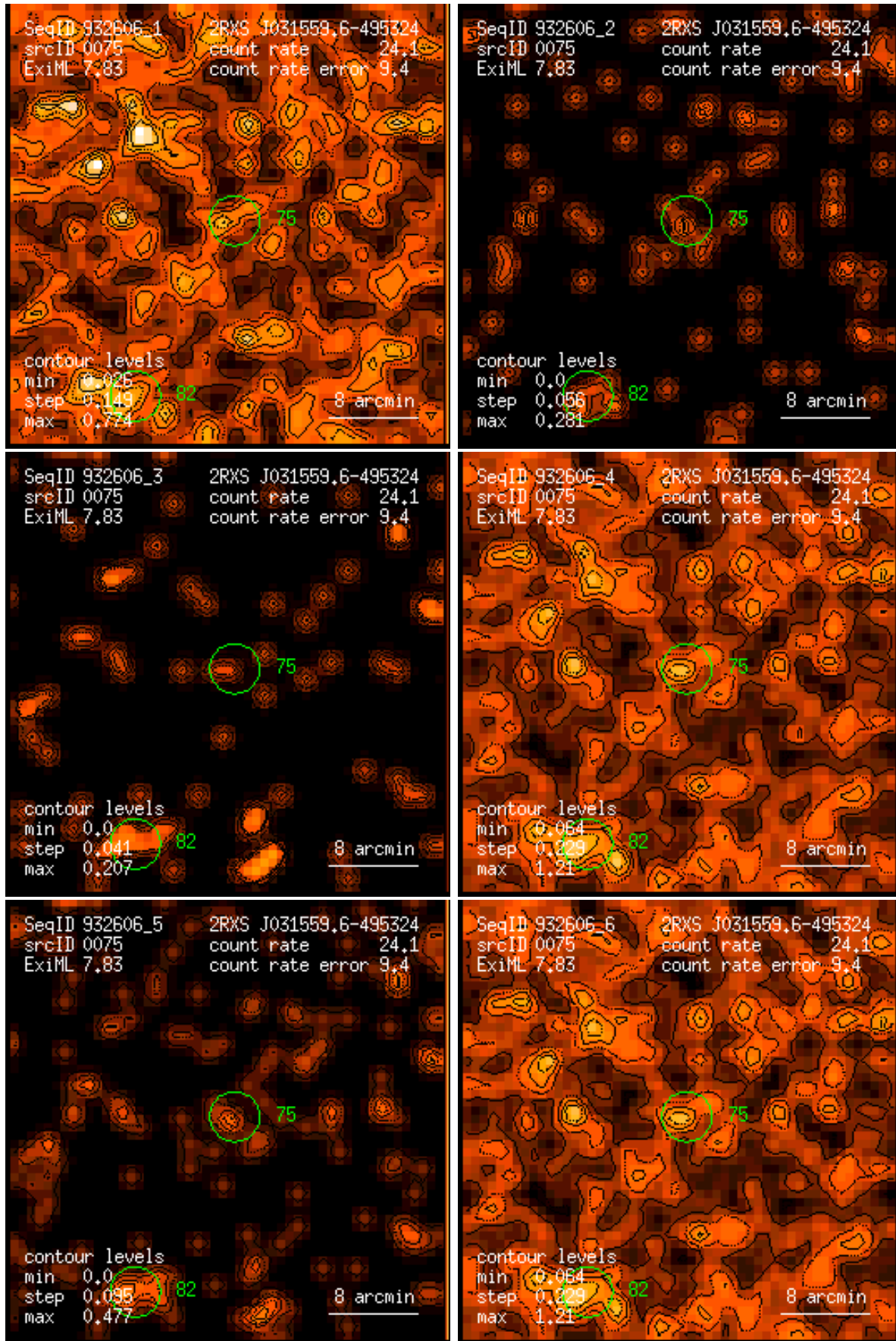
Figure 75: RASS 932606: detection 0075: band rate images, Gaussian filter: (1) PSPC channels 11 – 41, (2) 52 – 90, (3) 91 – 201, (4) 11 – 235, (5) 52 – 201, (6) 11 – 201. Broad band rates in counts/ks. Band rate contour levels in counts/ks/arcmin 2 .
