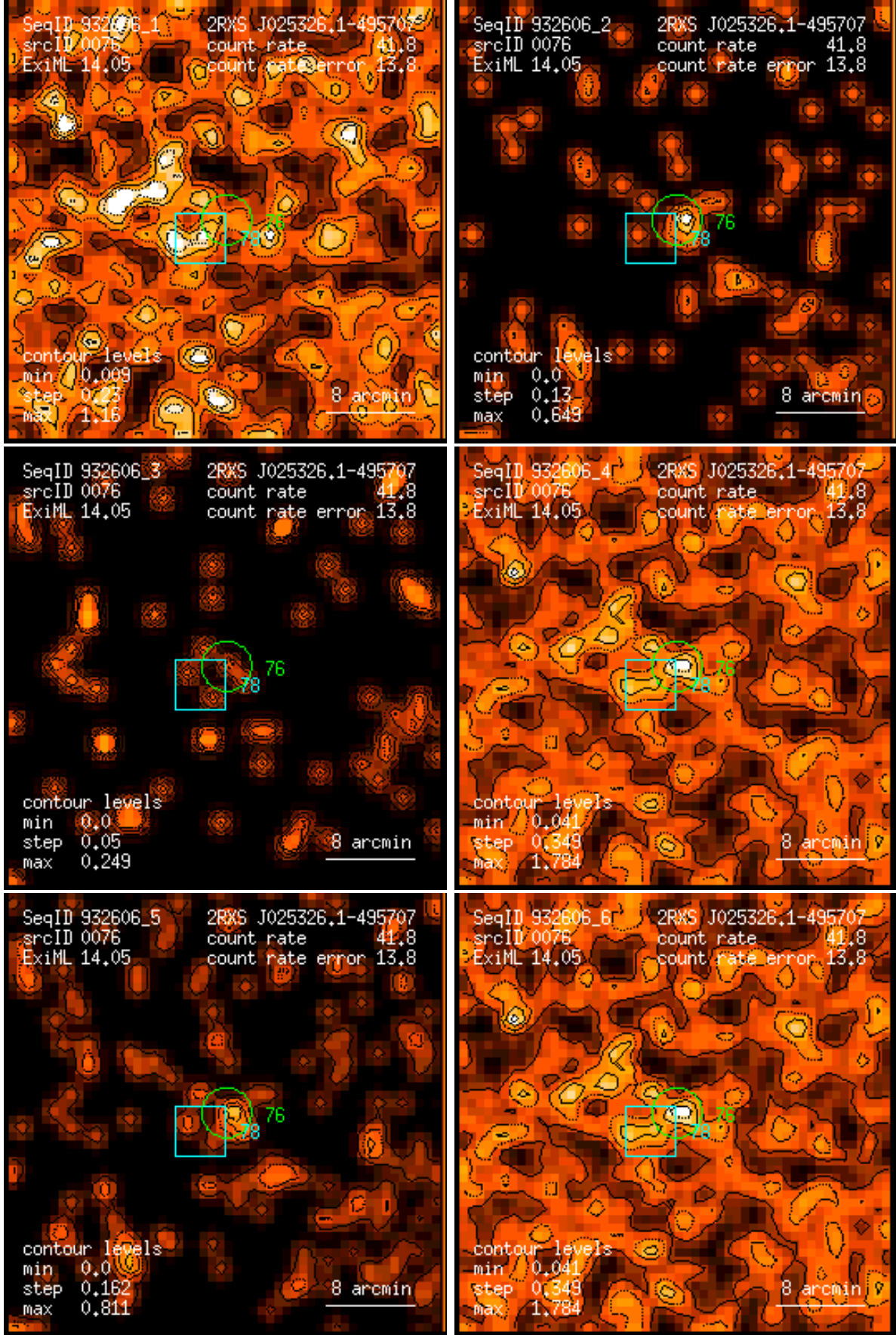
Figure 76: RASS 932606: detection 0076: band rate images, Gaussian filter: (1) PSPC channels 11 – 41, (2) 52 – 90, (3) 91 – 201, (4) 11 – 235, (5) 52 – 201, (6) 11 – 201. Broad band rates in counts/ks. Band rate contour levels in counts/ks/arcmin 2 .
