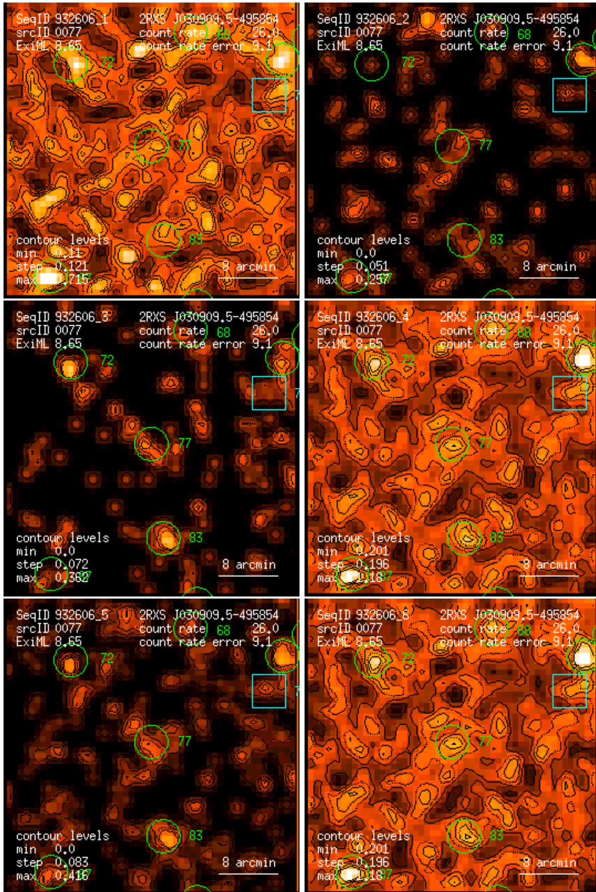
Figure 77: RASS 932606: detection 0077: band rate images, Gaussian filter: (1) PSPC channels 11 – 41, (2) 52 – 90, (3) 91 – 201, (4) 11 – 235, (5) 52 – 201, (6) 11 – 201. Broad band rates in counts/ks. Band rate contour levels in counts/ks/arcmin 2 .
