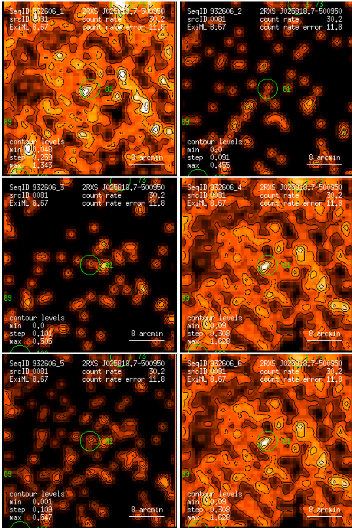
Figure 81: RASS 932606: detection 0081: band rate images, Gaussian filter: (1) PSPC channels 11 – 41, (2) 52 – 90, (3) 91 – 201, (4) 11 – 235, (5) 52 – 201, (6) 11 – 201. Broad band rates in counts/ks. Band rate contour levels in counts/ks/arcmin 2 .
