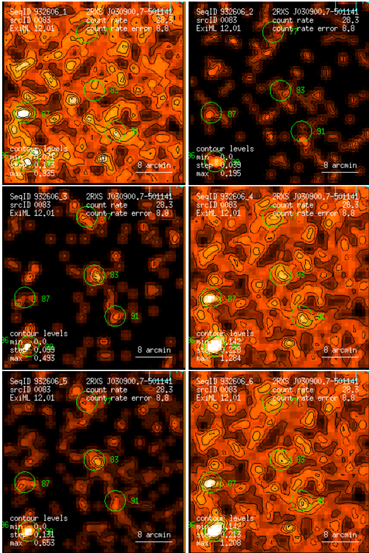
Figure 83: RASS 932606: detection 0083: band rate images, Gaussian filter: (1) PSPC channels 11 – 41, (2) 52 – 90, (3) 91 – 201, (4) 11 – 235, (5) 52 – 201, (6) 11 – 201. Broad band rates in counts/ks. Band rate contour levels in counts/ks/arcmin 2 .
