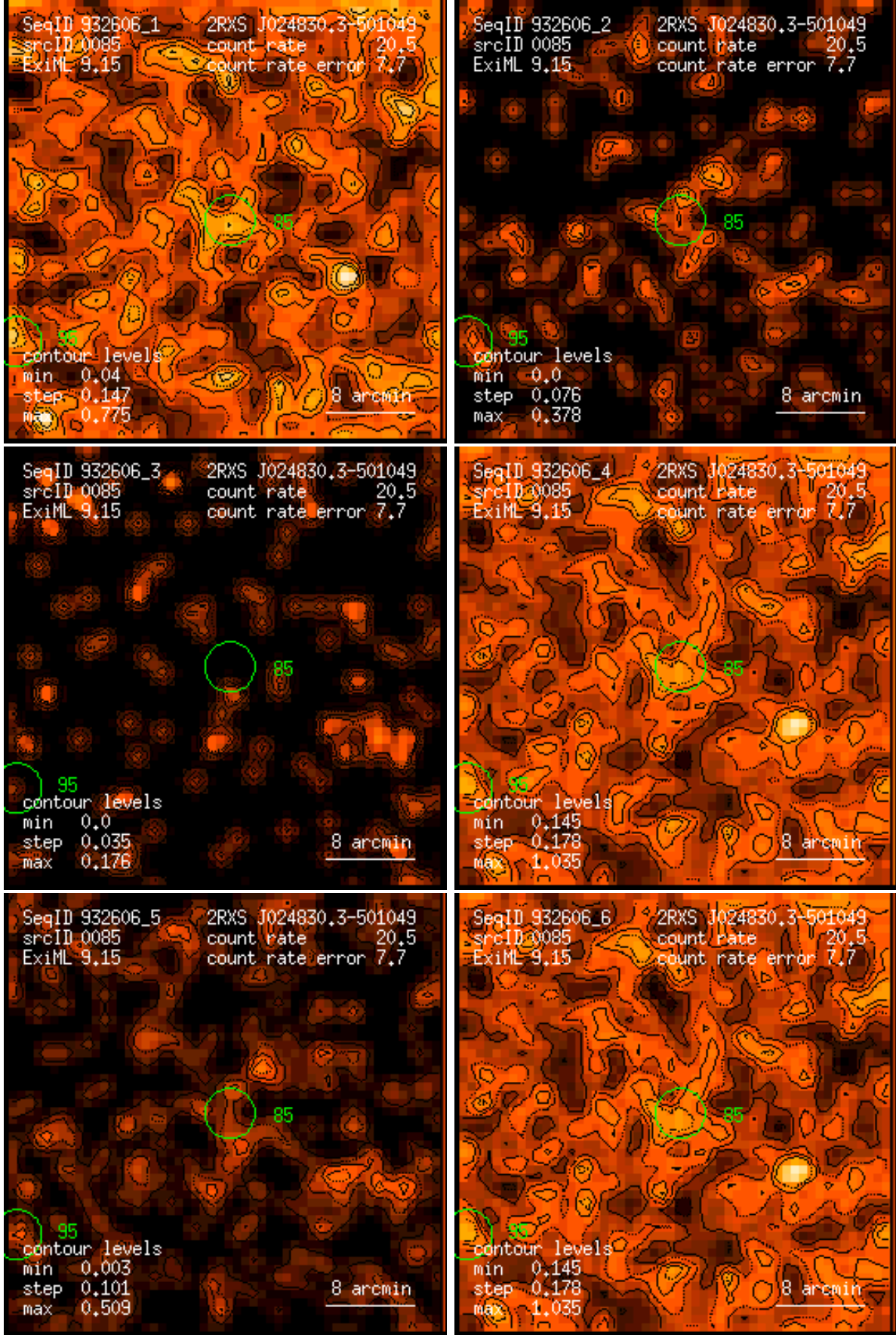
Figure 85: RASS 932606: detection 0085: band rate images, Gaussian filter: (1) PSPC channels 11 – 41, (2) 52 – 90, (3) 91 – 201, (4) 11 – 235, (5) 52 – 201, (6) 11 – 201. Broad band rates in counts/ks. Band rate contour levels in counts/ks/arcmin 2 .
