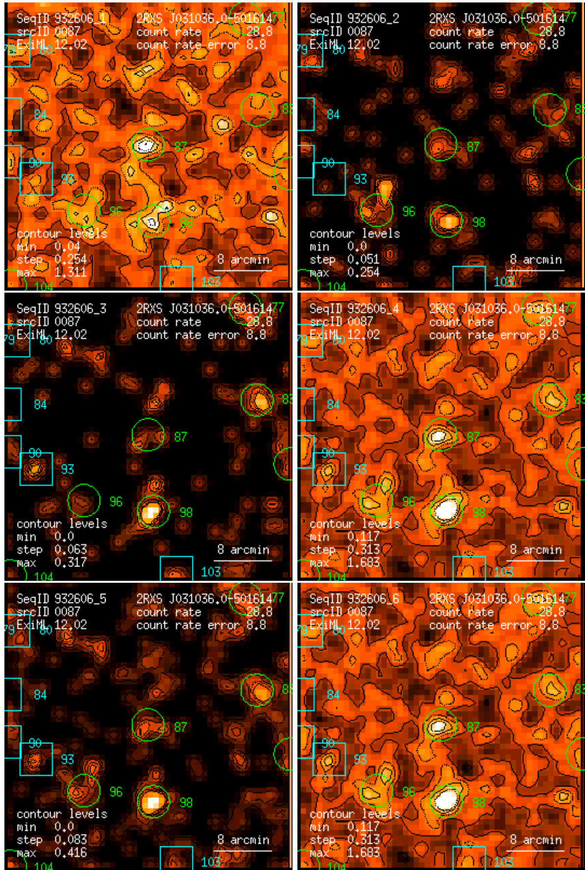
Figure 87: RASS 932606: detection 0087: band rate images, Gaussian filter: (1) PSPC channels 11 – 41, (2) 52 – 90, (3) 91 – 201, (4) 11 – 235, (5) 52 – 201, (6) 11 – 201. Broad band rates in counts/ks. Band rate contour levels in counts/ks/arcmin 2 .
