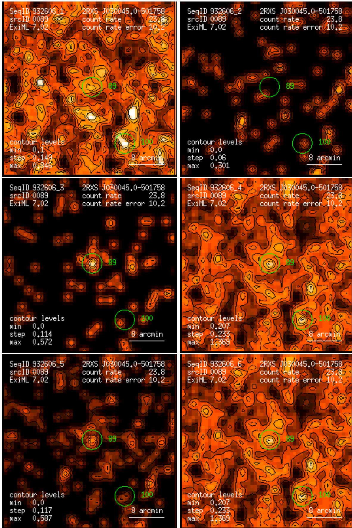
Figure 89: RASS 932606: detection 0089: band rate images, Gaussian filter: (1) PSPC channels 11 – 41, (2) 52 – 90, (3) 91 – 201, (4) 11 – 235, (5) 52 – 201, (6) 11 – 201. Broad band rates in counts/ks. Band rate contour levels in counts/ks/arcmin 2 .
