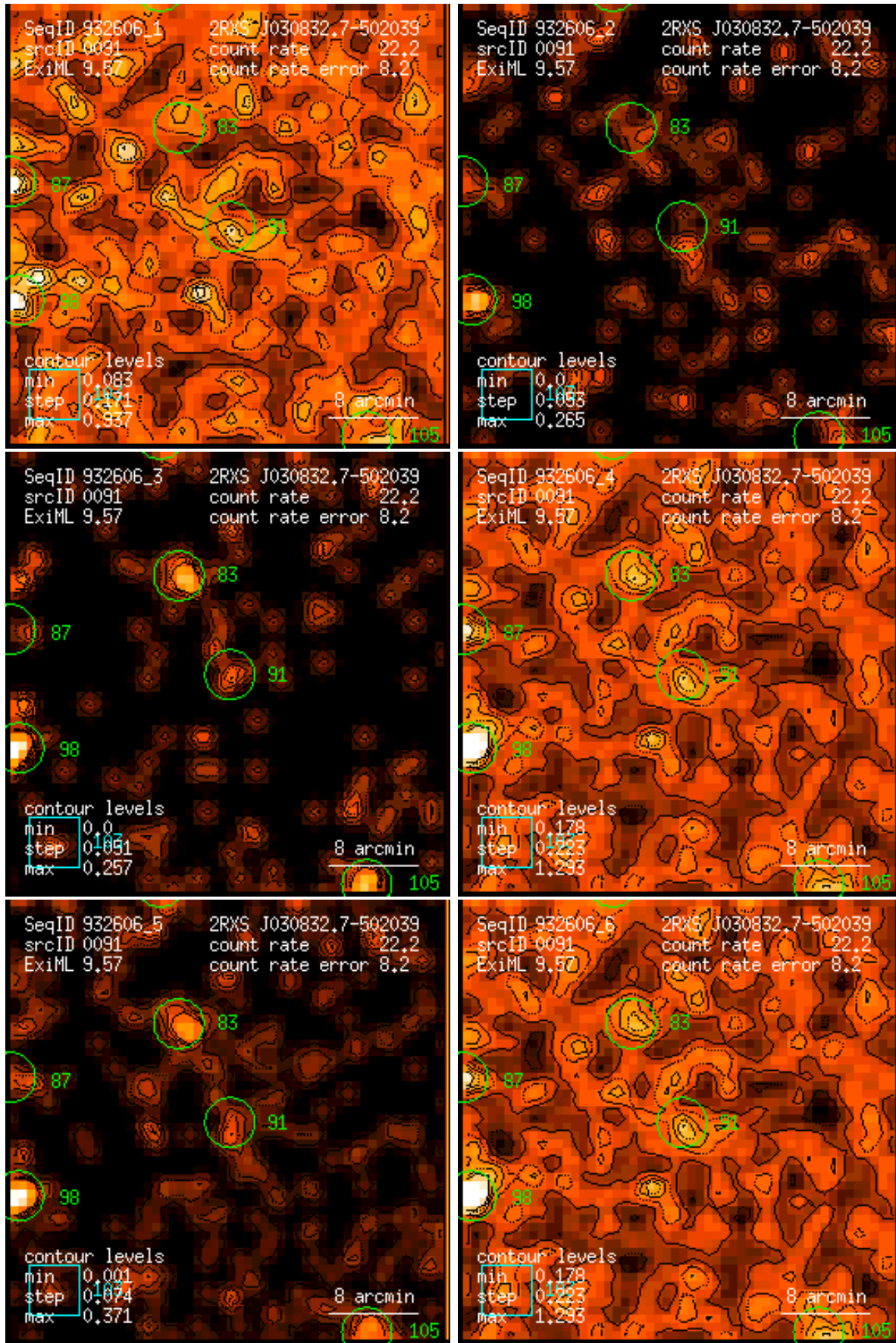
Figure 91: RASS 932606: detection 0091: band rate images, Gaussian filter: (1) PSPC channels 11 – 41, (2) 52 – 90, (3) 91 – 201, (4) 11 – 235, (5) 52 – 201, (6) 11 – 201. Broad band rates in counts/ks. Band rate contour levels in counts/ks/arcmin 2 .
