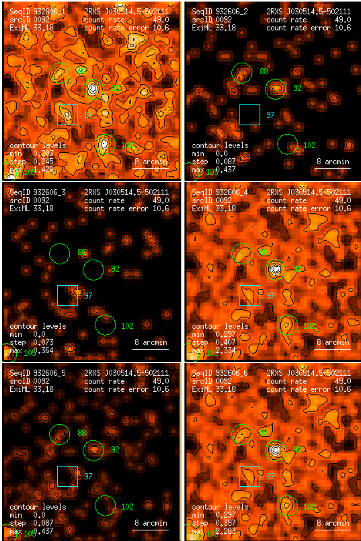
Figure 92: RASS 932606: detection 0092: band rate images, Gaussian filter: (1) PSPC channels 11 – 41, (2) 52 – 90, (3) 91 – 201, (4) 11 – 235, (5) 52 – 201, (6) 11 – 201. Broad band rates in counts/ks. Band rate contour levels in counts/ks/arcmin 2 .
