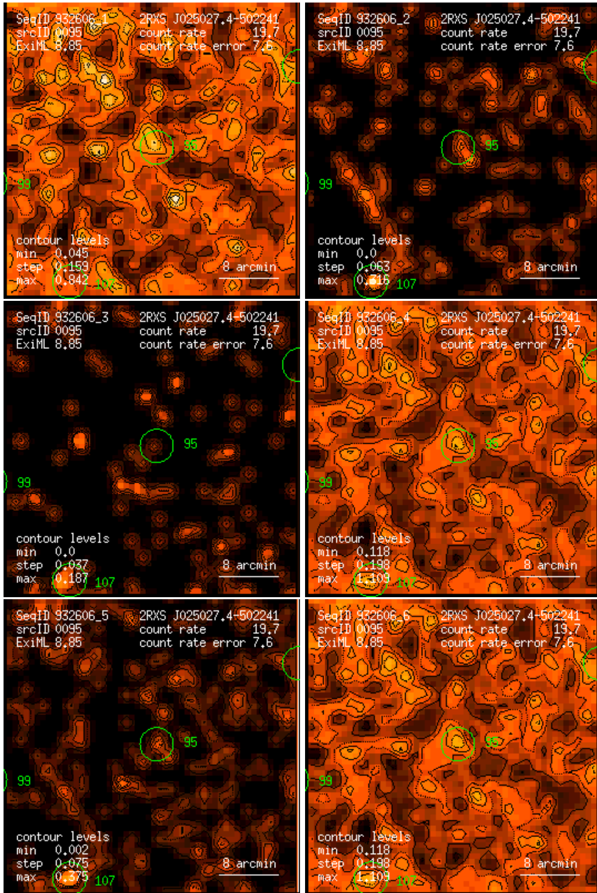
Figure 95: RASS 932606: detection 0095: band rate images, Gaussian filter: (1) PSPC channels 11 – 41, (2) 52 – 90, (3) 91 – 201, (4) 11 – 235, (5) 52 – 201, (6) 11 – 201. Broad band rates in counts/ks. Band rate contour levels in counts/ks/arcmin 2 .
