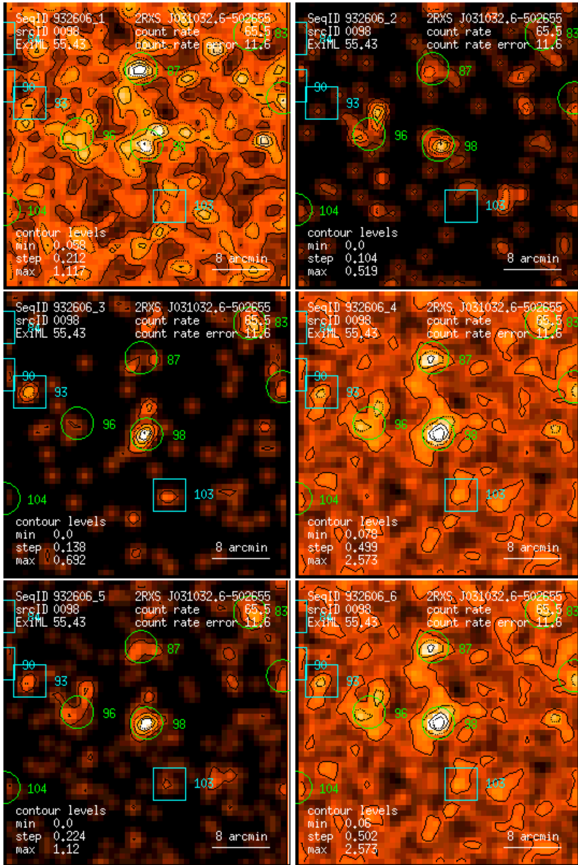
Figure 98: RASS 932606: detection 0098: band rate images, Gaussian filter: (1) PSPC channels 11 – 41, (2) 52 – 90, (3) 91 – 201, (4) 11 – 235, (5) 52 – 201, (6) 11 – 201. Broad band rates in counts/ks. Band rate contour levels in counts/ks/arcmin 2 .
