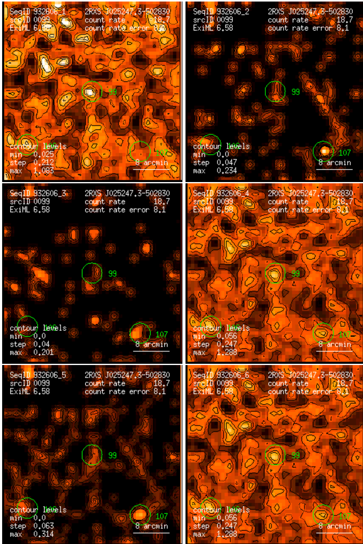
Figure 99: RASS 932606: detection 0099: band rate images, Gaussian filter: (1) PSPC channels 11 – 41, (2) 52 – 90, (3) 91 – 201, (4) 11 – 235, (5) 52 – 201, (6) 11 – 201. Broad band rates in counts/ks. Band rate contour levels in counts/ks/arcmin 2 .
