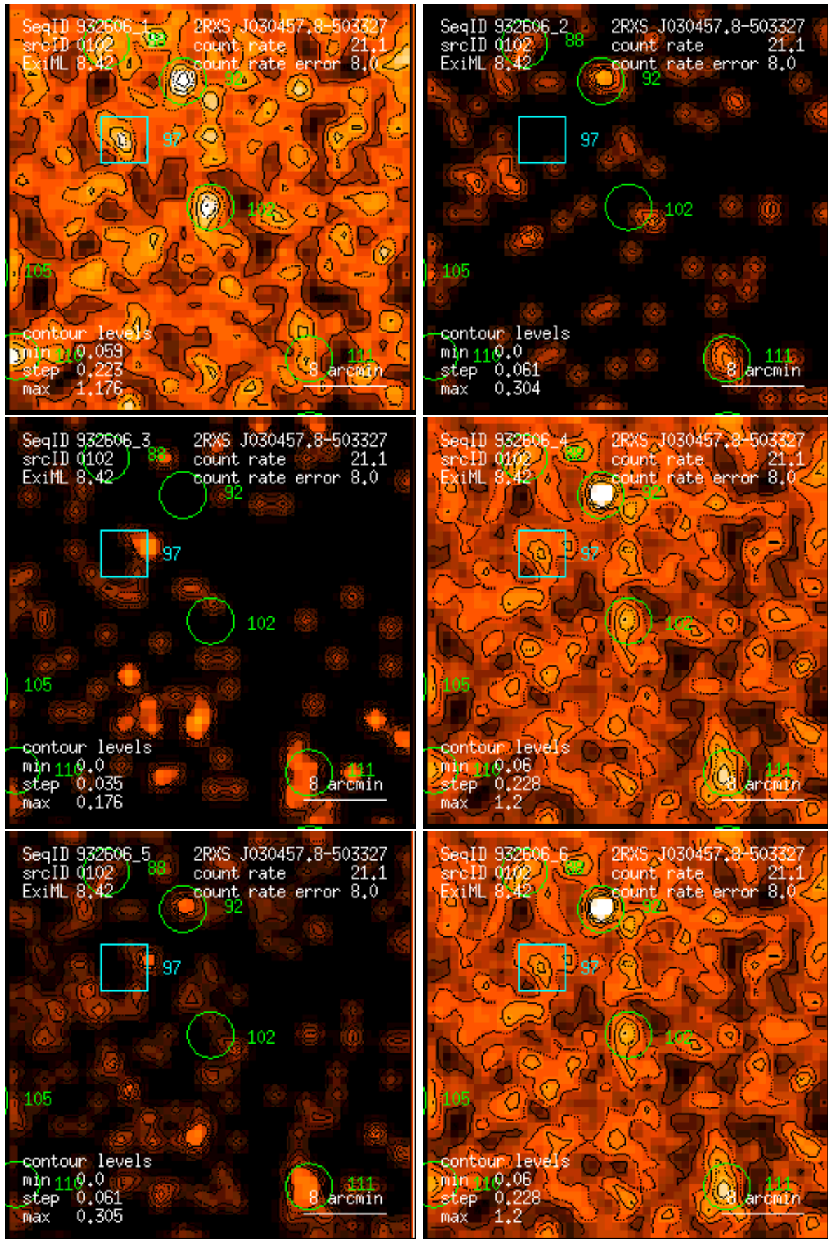
Figure 102: RASS 932606: detection 0102: band rate images, Gaussian filter: (1) PSPC channels 11 – 41, (2) 52 – 90, (3) 91 – 201, (4) 11 – 235, (5) 52 – 201, (6) 11 – 201. Broad band rates in counts/ks. Band rate contour levels in counts/ks/arcmin 2 .
