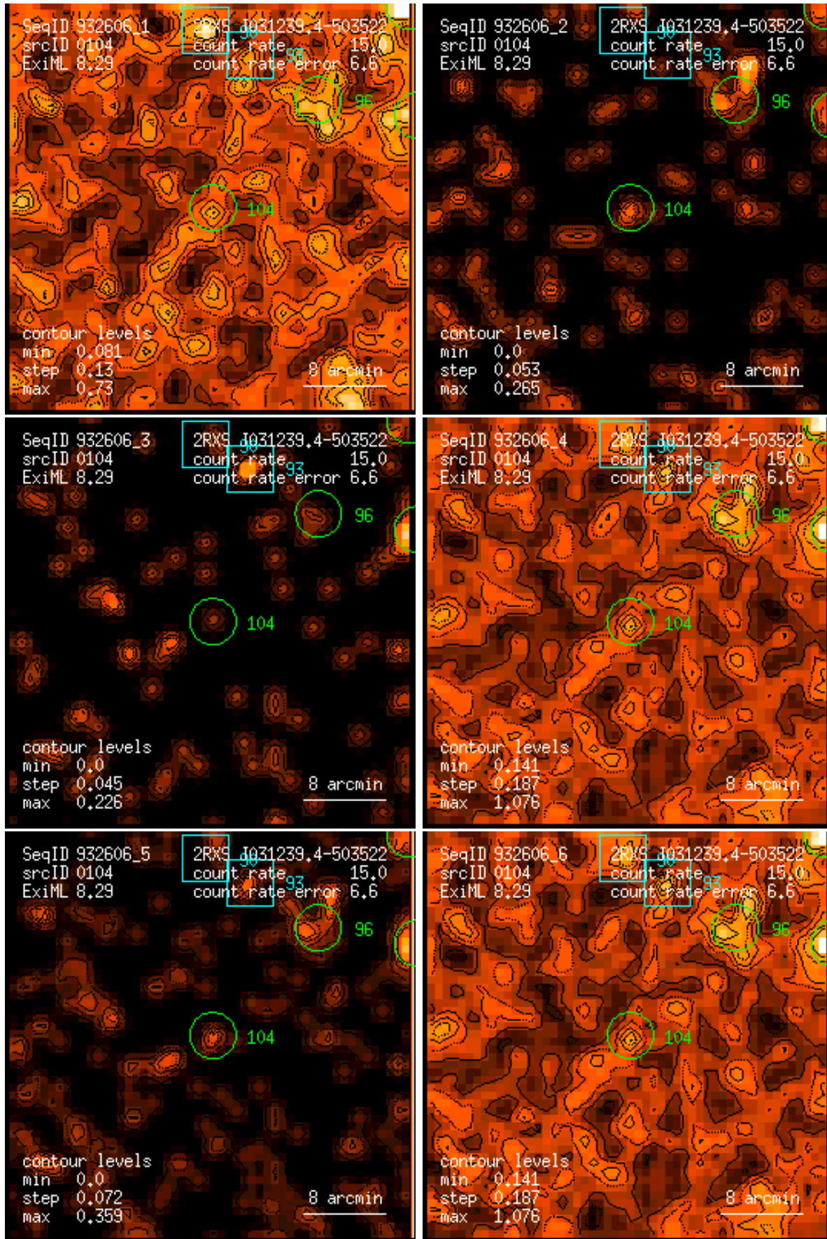
Figure 104: RASS 932606: detection 0104: band rate images, Gaussian filter: (1) PSPC channels 11 – 41, (2) 52 – 90, (3) 91 – 201, (4) 11 – 235, (5) 52 – 201, (6) 11 – 201. Broad band rates in counts/ks. Band rate contour levels in counts/ks/arcmin 2 .
