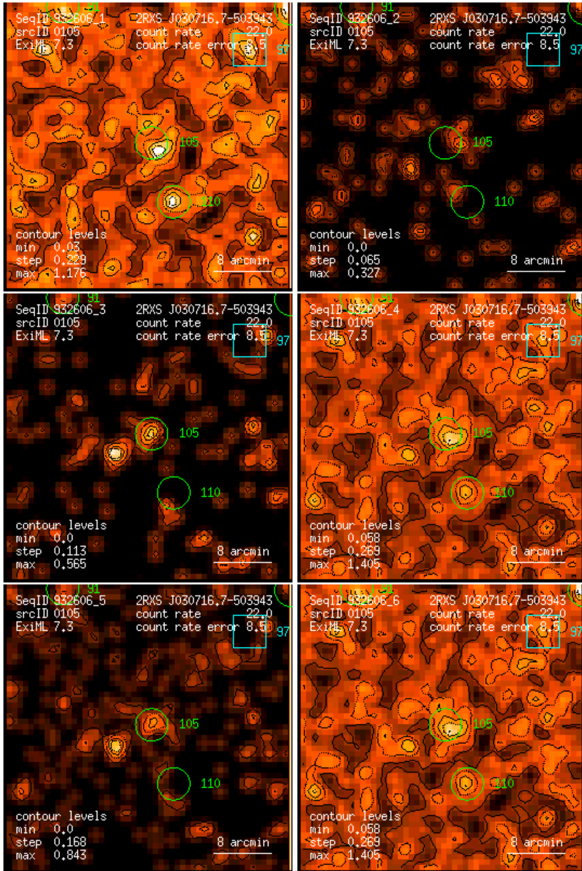
Figure 105: RASS 932606: detection 0105: band rate images, Gaussian filter: (1) PSPC channels 11 – 41, (2) 52 – 90, (3) 91 – 201, (4) 11 – 235, (5) 52 – 201, (6) 11 – 201. Broad band rates in counts/ks. Band rate contour levels in counts/ks/arcmin 2 .
