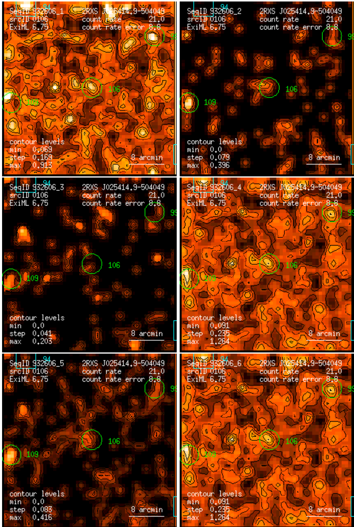
Figure 106: RASS 932606: detection 0106: band rate images, Gaussian filter: (1) PSPC channels 11 – 41, (2) 52 – 90, (3) 91 – 201, (4) 11 – 235, (5) 52 – 201, (6) 11 – 201. Broad band rates in counts/ks. Band rate contour levels in counts/ks/arcmin 2 .
