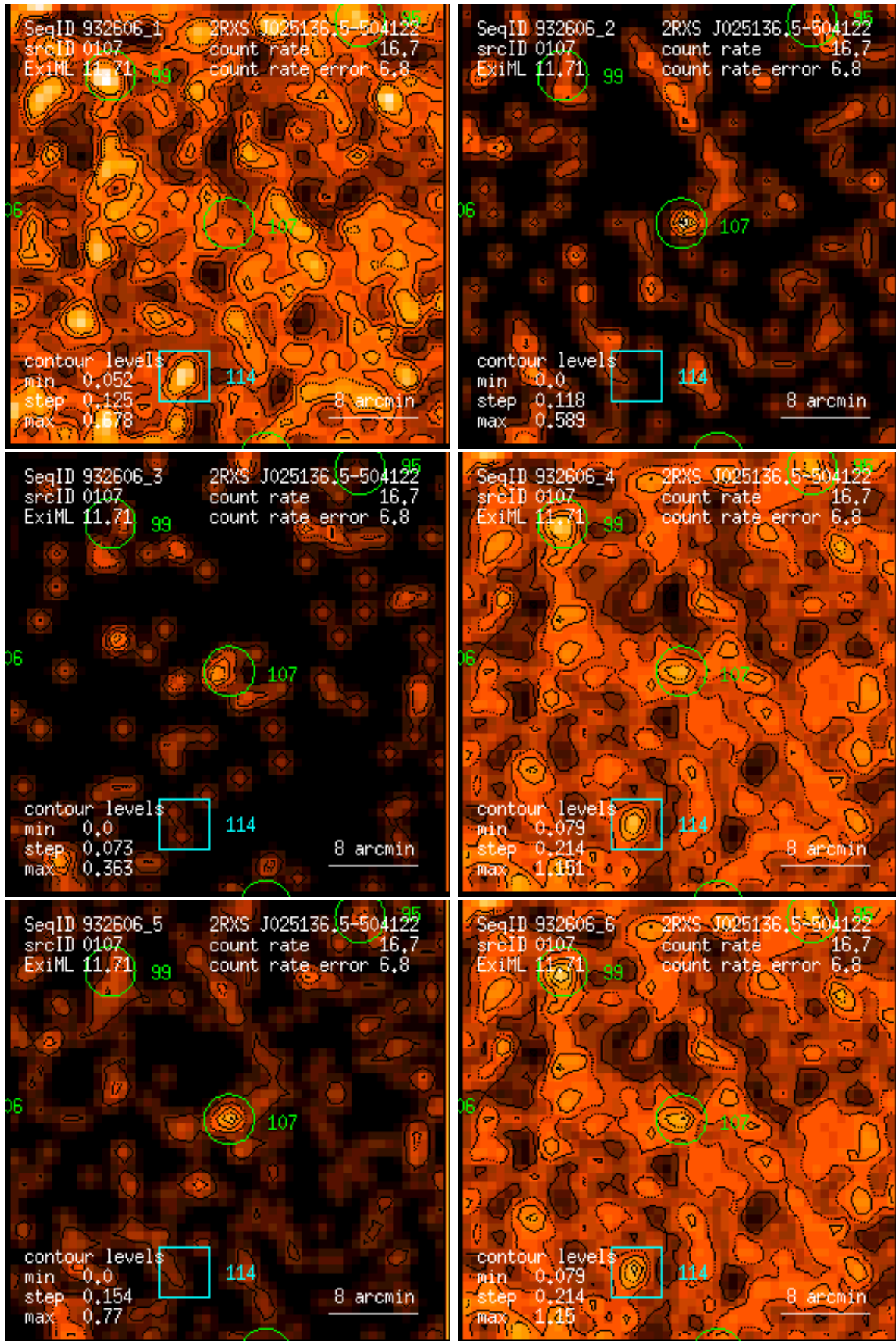
Figure 107: RASS 932606: detection 0107: band rate images, Gaussian filter: (1) PSPC channels 11 – 41, (2) 52 – 90, (3) 91 – 201, (4) 11 – 235, (5) 52 – 201, (6) 11 – 201. Broad band rates in counts/ks. Band rate contour levels in counts/ks/arcmin 2 .
