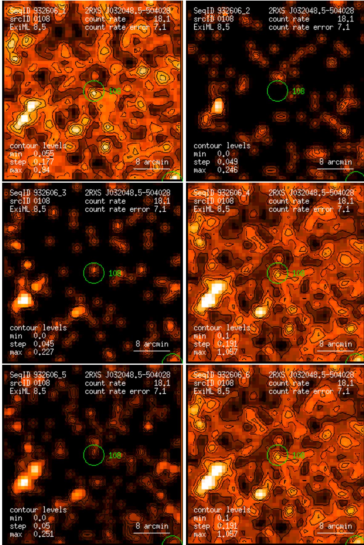
Figure 108: RASS 932606: detection 0108: band rate images, Gaussian filter: (1) PSPC channels 11 – 41, (2) 52 – 90, (3) 91 – 201, (4) 11 – 235, (5) 52 – 201, (6) 11 – 201. Broad band rates in counts/ks. Band rate contour levels in counts/ks/arcmin 2 .
