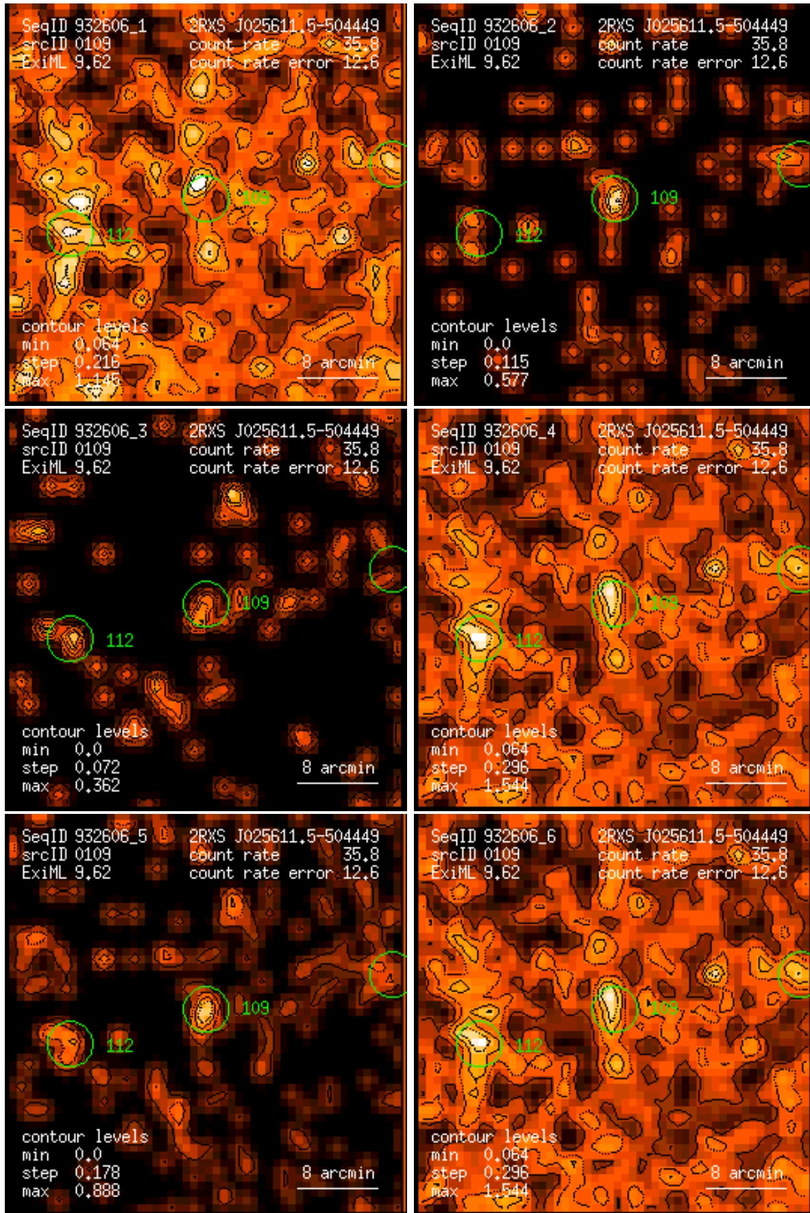
Figure 109: RASS 932606: detection 0109: band rate images, Gaussian filter: (1) PSPC channels 11 – 41, (2) 52 – 90, (3) 91 – 201, (4) 11 – 235, (5) 52 – 201, (6) 11 – 201. Broad band rates in counts/ks. Band rate contour levels in counts/ks/arcmin 2 .
