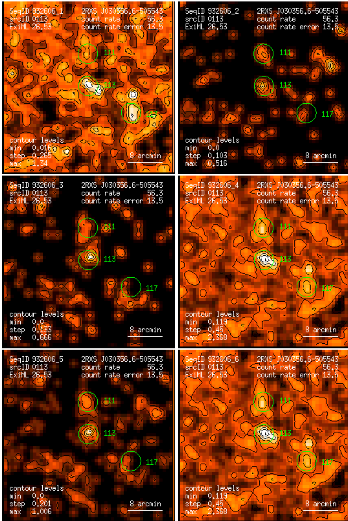
Figure 113: RASS 932606: detection 0113: band rate images, Gaussian filter: (1) PSPC channels 11 – 41, (2) 52 – 90, (3) 91 – 201, (4) 11 – 235, (5) 52 – 201, (6) 11 – 201. Broad band rates in counts/ks. Band rate contour levels in counts/ks/arcmin 2 .
