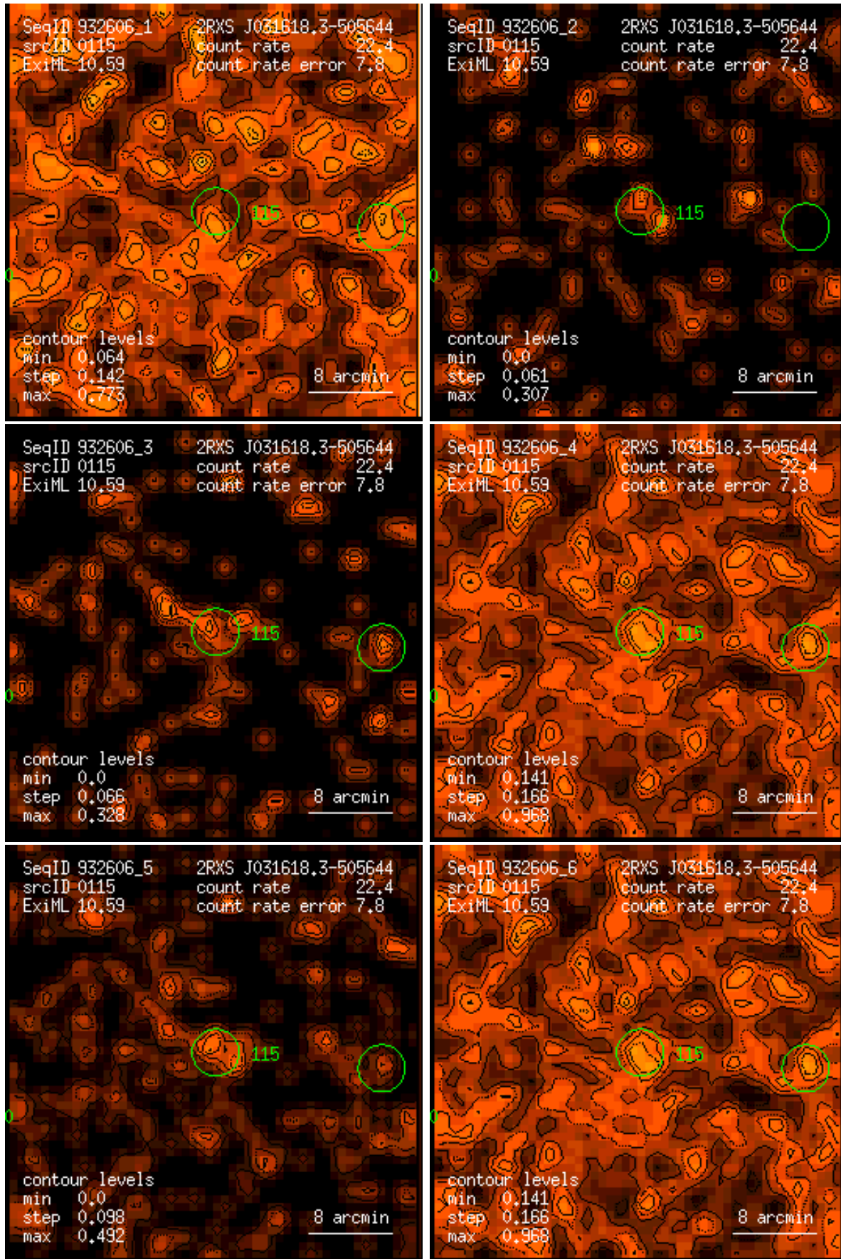
Figure 115: RASS 932606: detection 0115: band rate images, Gaussian filter: (1) PSPC channels 11 – 41, (2) 52 – 90, (3) 91 – 201, (4) 11 – 235, (5) 52 – 201, (6) 11 – 201. Broad band rates in counts/ks. Band rate contour levels in counts/ks/arcmin 2 .
