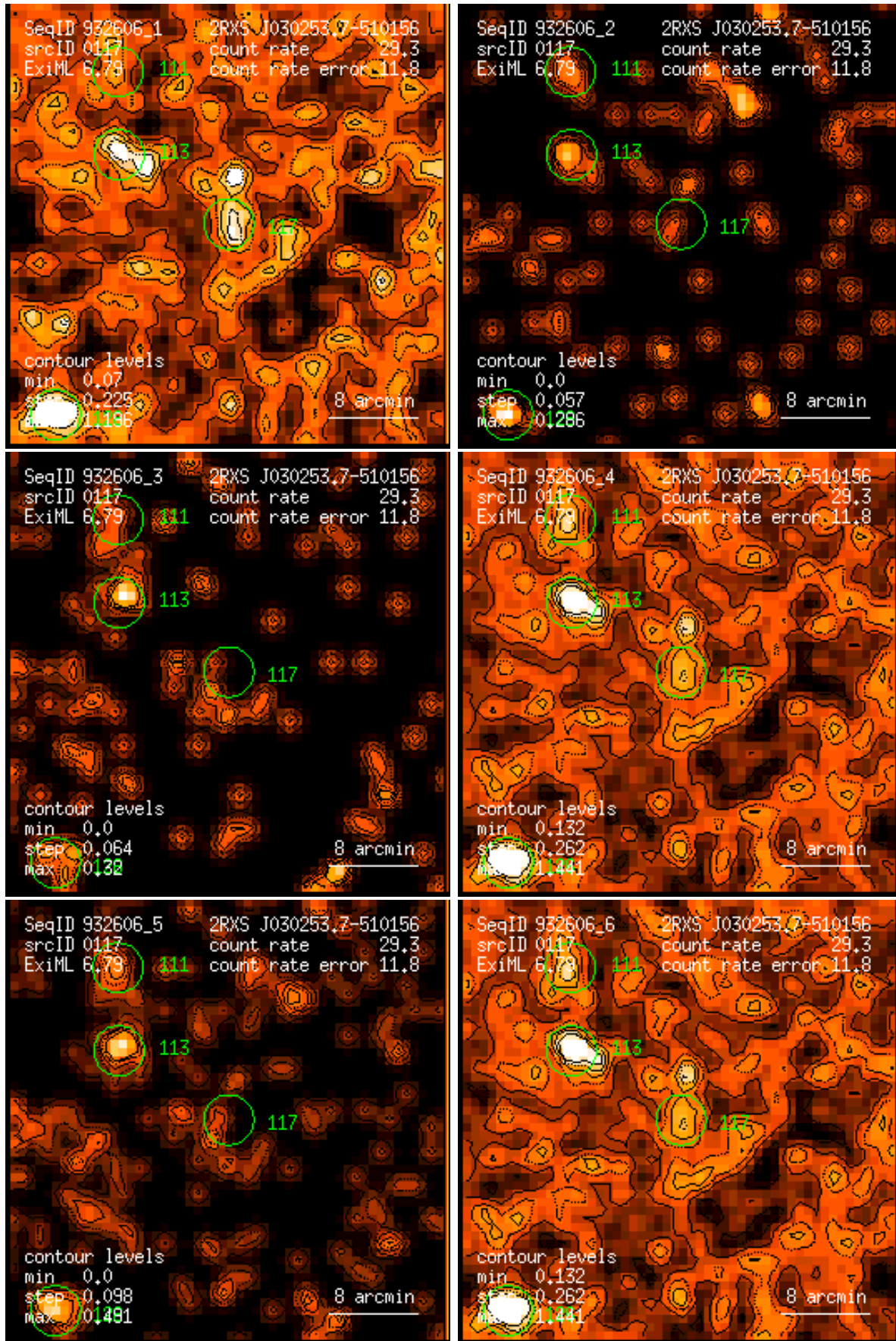
Figure 117: RASS 932606: detection 0117: band rate images, Gaussian filter: (1) PSPC channels 11 – 41, (2) 52 – 90, (3) 91 – 201, (4) 11 – 235, (5) 52 – 201, (6) 11 – 201. Broad band rates in counts/ks. Band rate contour levels in counts/ks/arcmin 2 .
