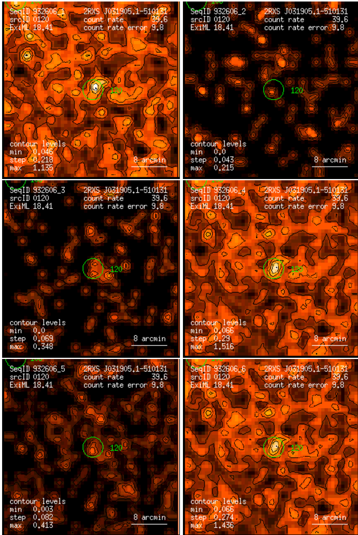
Figure 120: RASS 932606: detection 0120: band rate images, Gaussian filter: (1) PSPC channels 11 – 41, (2) 52 – 90, (3) 91 – 201, (4) 11 – 235, (5) 52 – 201, (6) 11 – 201. Broad band rates in counts/ks. Band rate contour levels in counts/ks/arcmin 2 .
