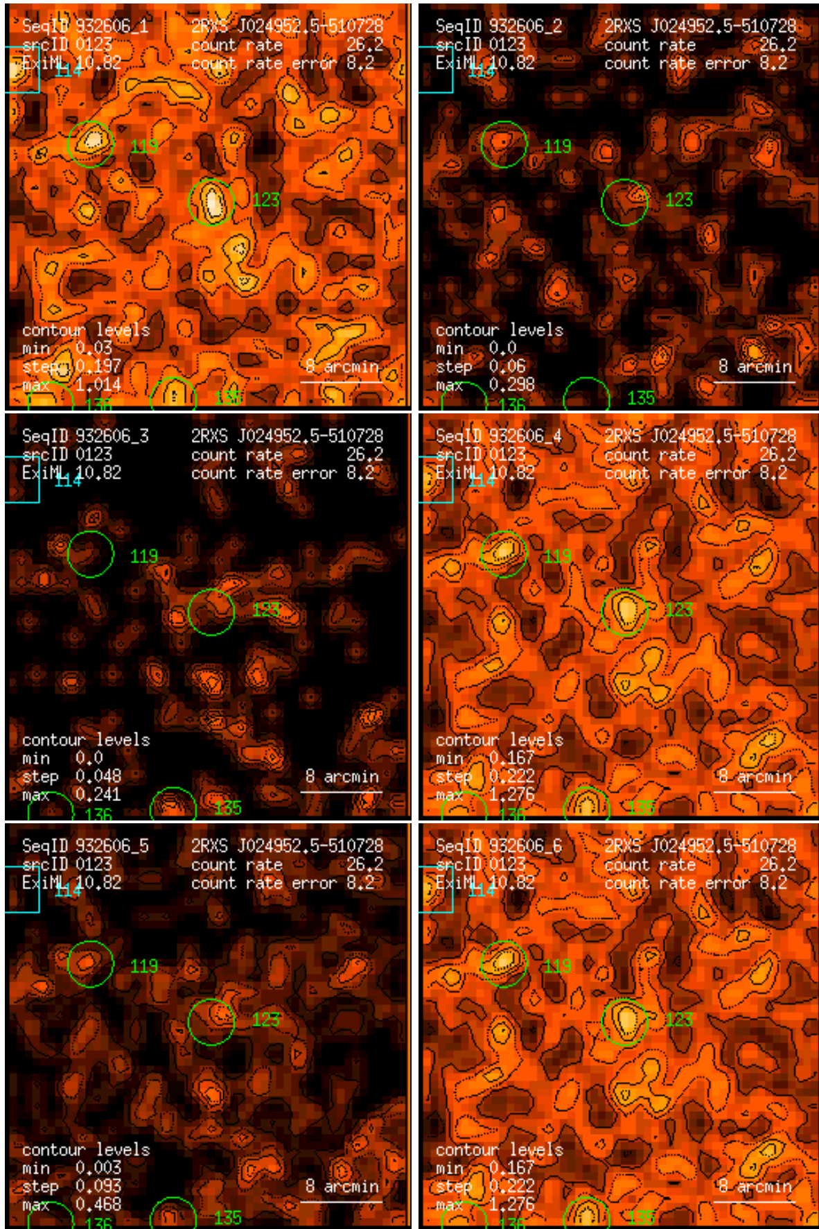
Figure 123: RASS 932606: detection 0123: band rate images, Gaussian filter: (1) PSPC channels 11 – 41, (2) 52 – 90, (3) 91 – 201, (4) 11 – 235, (5) 52 – 201, (6) 11 – 201. Broad band rates in counts/ks. Band rate contour levels in counts/ks/arcmin 2 .
