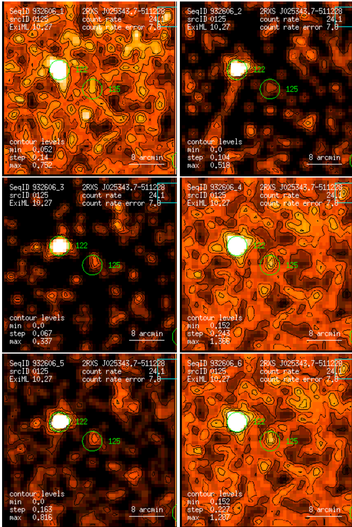
Figure 125: RASS 932606: detection 0125: band rate images, Gaussian filter: (1) PSPC channels 11 – 41, (2) 52 – 90, (3) 91 – 201, (4) 11 – 235, (5) 52 – 201, (6) 11 – 201. Broad band rates in counts/ks. Band rate contour levels in counts/ks/arcmin 2 .
