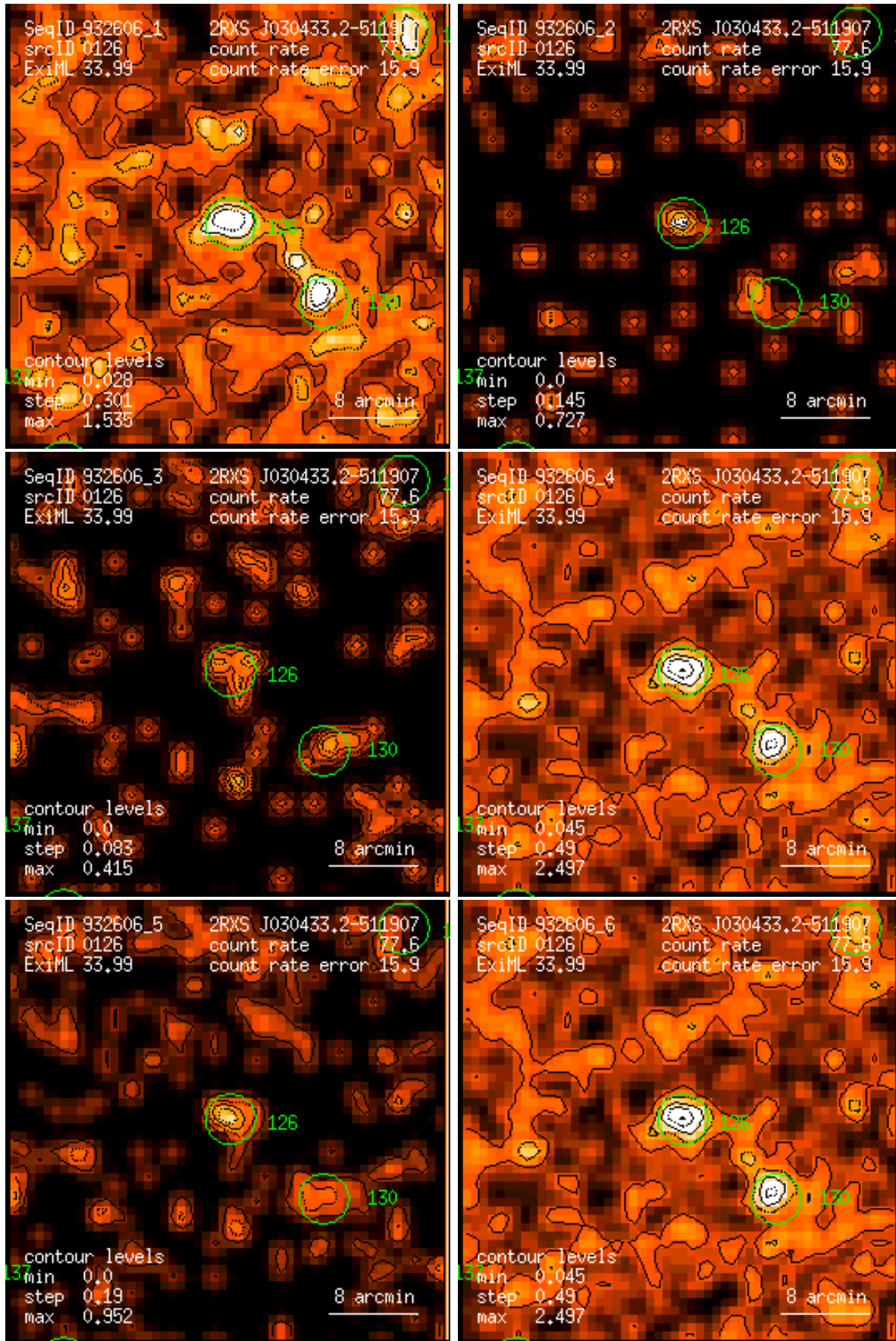
Figure 126: RASS 932606: detection 0126: band rate images, Gaussian filter: (1) PSPC channels 11 – 41, (2) 52 – 90, (3) 91 – 201, (4) 11 – 235, (5) 52 – 201, (6) 11 – 201. Broad band rates in counts/ks. Band rate contour levels in counts/ks/arcmin 2 .
