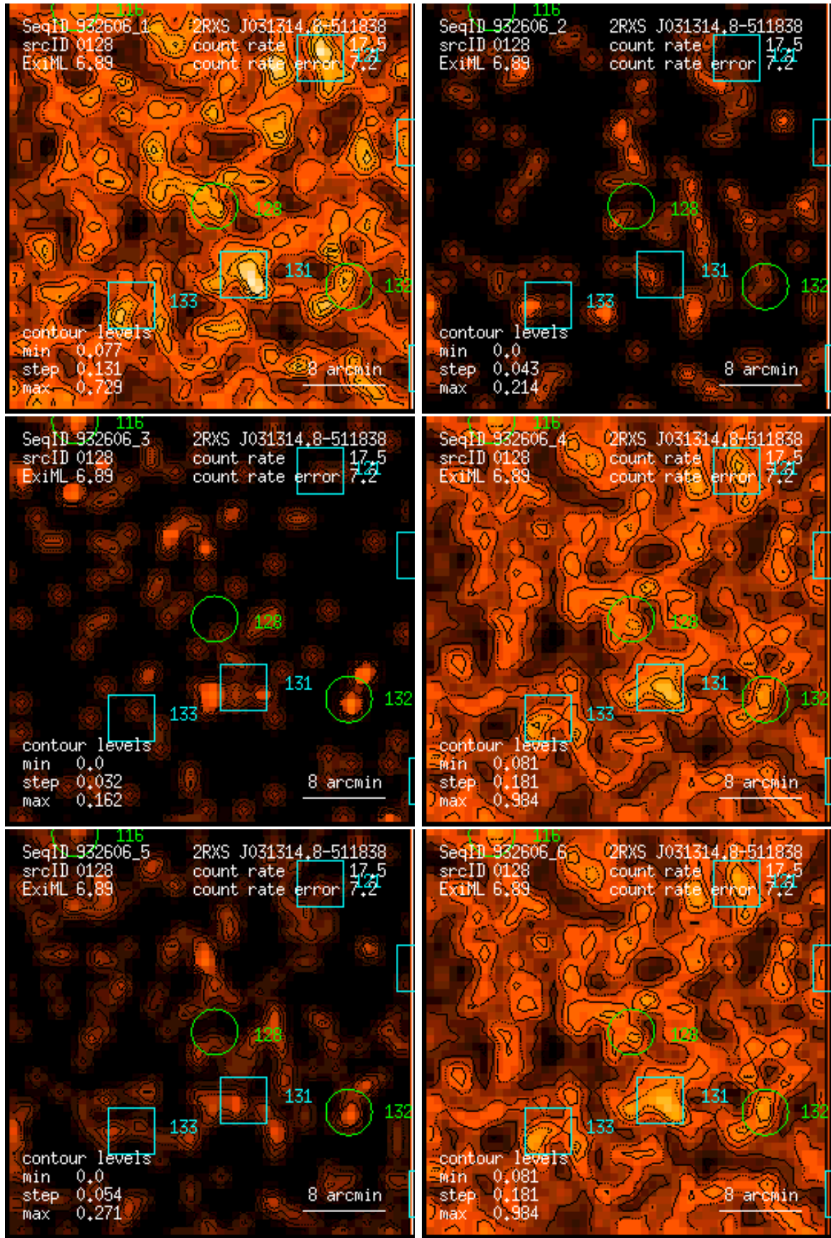
Figure 128: RASS 932606: detection 0128: band rate images, Gaussian filter: (1) PSPC channels 11 – 41, (2) 52 – 90, (3) 91 – 201, (4) 11 – 235, (5) 52 – 201, (6) 11 – 201. Broad band rates in counts/ks. Band rate contour levels in counts/ks/arcmin 2 .
