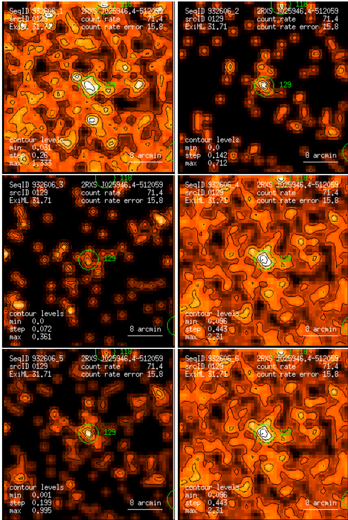
Figure 129: RASS 932606: detection 0129: band rate images, Gaussian filter: (1) PSPC channels 11 – 41, (2) 52 – 90, (3) 91 – 201, (4) 11 – 235, (5) 52 – 201, (6) 11 – 201. Broad band rates in counts/ks. Band rate contour levels in counts/ks/arcmin 2 .
