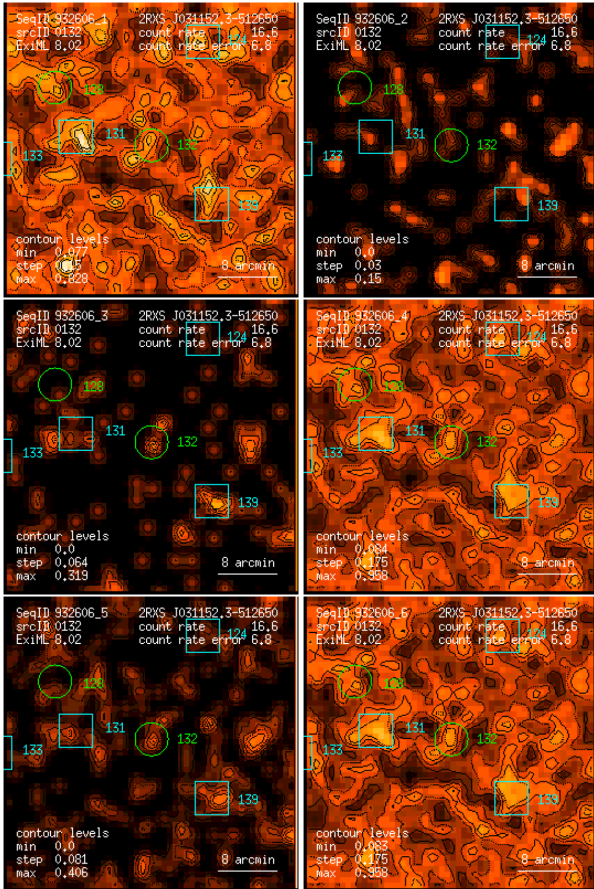
Figure 132: RASS 932606: detection 0132: band rate images, Gaussian filter: (1) PSPC channels 11 – 41, (2) 52 – 90, (3) 91 – 201, (4) 11 – 235, (5) 52 – 201, (6) 11 – 201. Broad band rates in counts/ks. Band rate contour levels in counts/ks/arcmin 2 .
