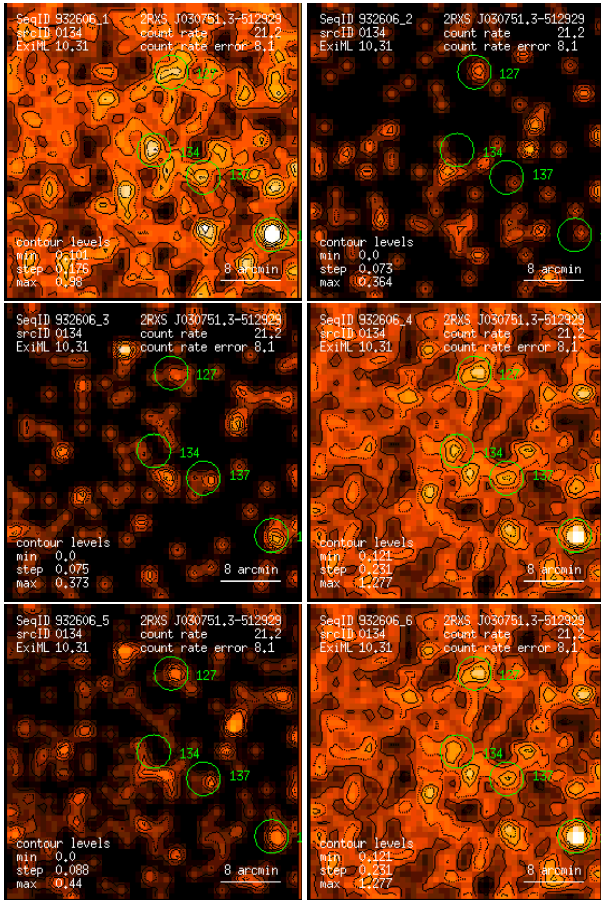
Figure 134: RASS 932606: detection 0134: band rate images, Gaussian filter: (1) PSPC channels 11 – 41, (2) 52 – 90, (3) 91 – 201, (4) 11 – 235, (5) 52 – 201, (6) 11 – 201. Broad band rates in counts/ks. Band rate contour levels in counts/ks/arcmin 2 .
