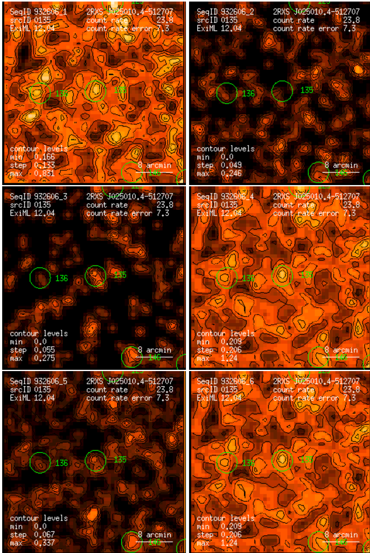
Figure 135: RASS 932606: detection 0135: band rate images, Gaussian filter: (1) PSPC channels 11 – 41, (2) 52 – 90, (3) 91 – 201, (4) 11 – 235, (5) 52 – 201, (6) 11 – 201. Broad band rates in counts/ks. Band rate contour levels in counts/ks/arcmin 2 .
