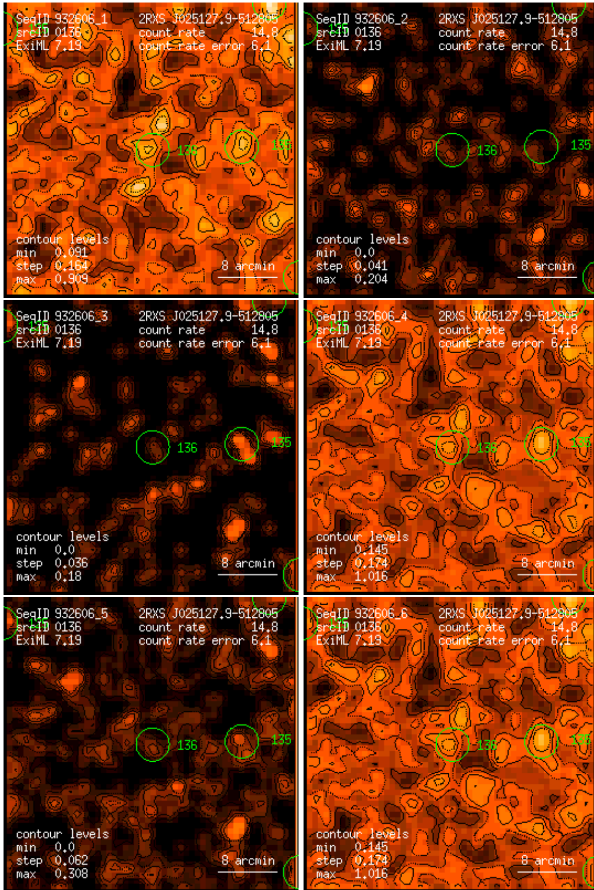
Figure 136: RASS 932606: detection 0136: band rate images, Gaussian filter: (1) PSPC channels 11 – 41, (2) 52 – 90, (3) 91 – 201, (4) 11 – 235, (5) 52 – 201, (6) 11 – 201. Broad band rates in counts/ks. Band rate contour levels in counts/ks/arcmin 2 .
