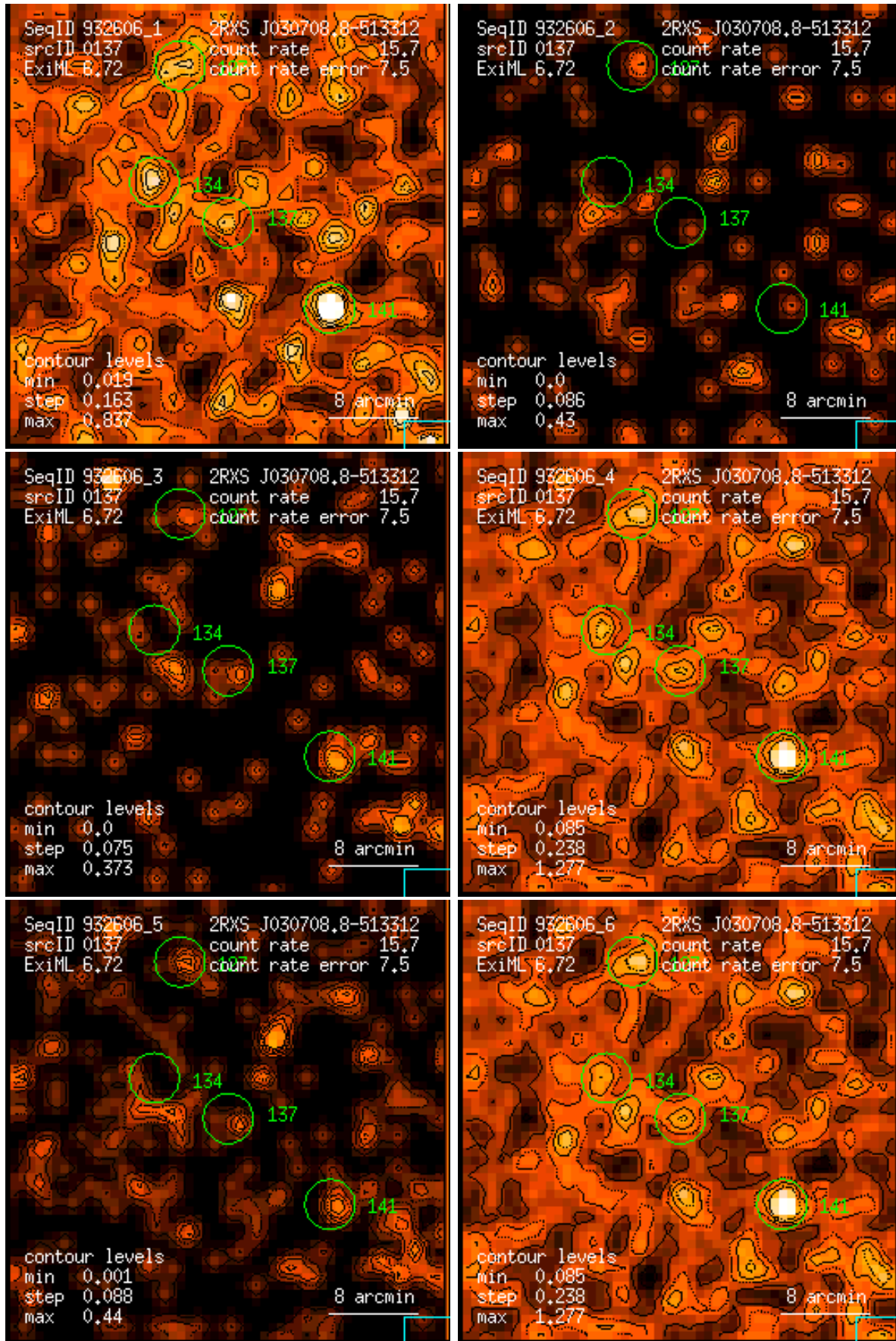
Figure 137: RASS 932606: detection 0137: band rate images, Gaussian filter: (1) PSPC channels 11 – 41, (2) 52 – 90, (3) 91 – 201, (4) 11 – 235, (5) 52 – 201, (6) 11 – 201. Broad band rates in counts/ks. Band rate contour levels in counts/ks/arcmin 2 .
