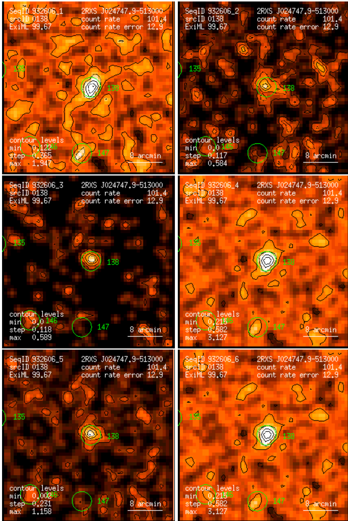
Figure 138: RASS 932606: detection 0138: band rate images, Gaussian filter: (1) PSPC channels 11 – 41, (2) 52 – 90, (3) 91 – 201, (4) 11 – 235, (5) 52 – 201, (6) 11 – 201. Broad band rates in counts/ks. Band rate contour levels in counts/ks/arcmin 2 .
