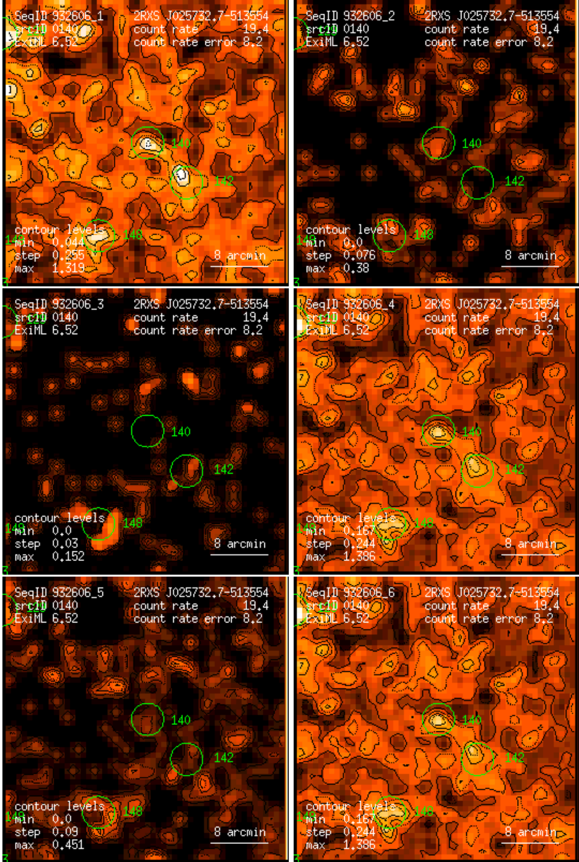
Figure 140: RASS 932606: detection 0140: band rate images, Gaussian filter: (1) PSPC channels 11 – 41, (2) 52 – 90, (3) 91 – 201, (4) 11 – 235, (5) 52 – 201, (6) 11 – 201. Broad band rates in counts/ks. Band rate contour levels in counts/ks/arcmin 2 .
