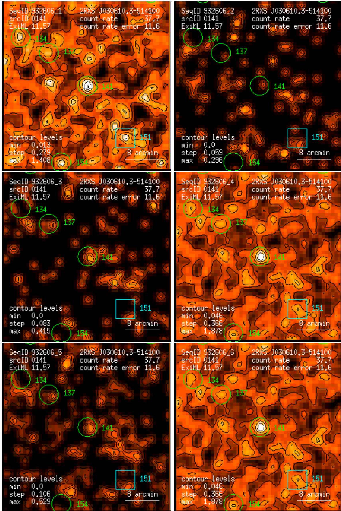
Figure 141: RASS 932606: detection 0141: band rate images, Gaussian filter: (1) PSPC channels 11 – 41, (2) 52 – 90, (3) 91 – 201, (4) 11 – 235, (5) 52 – 201, (6) 11 – 201. Broad band rates in counts/ks. Band rate contour levels in counts/ks/arcmin 2 .
