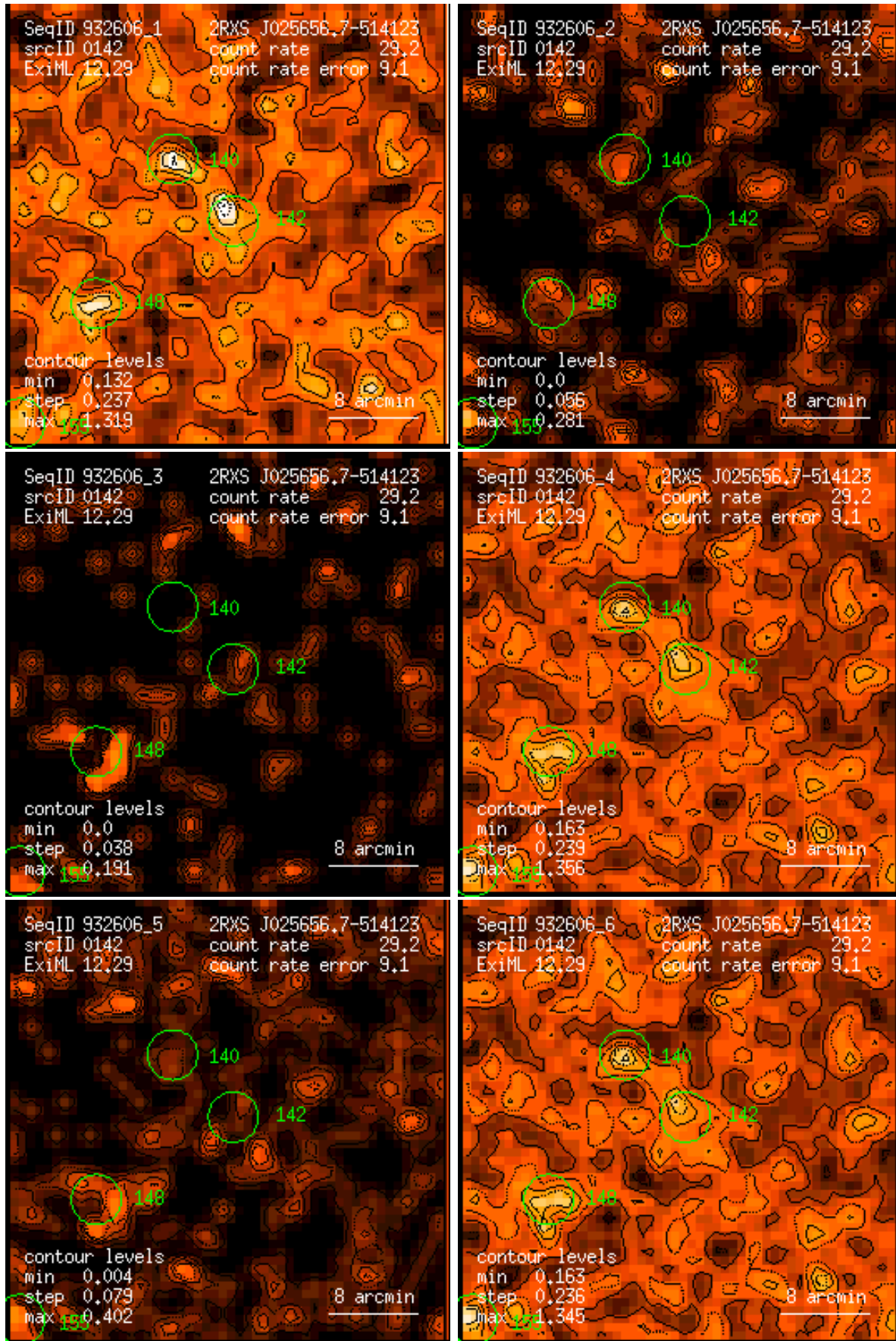
Figure 142: RASS 932606: detection 0142: band rate images, Gaussian filter: (1) PSPC channels 11 – 41, (2) 52 – 90, (3) 91 – 201, (4) 11 – 235, (5) 52 – 201, (6) 11 – 201. Broad band rates in counts/ks. Band rate contour levels in counts/ks/arcmin 2 .
