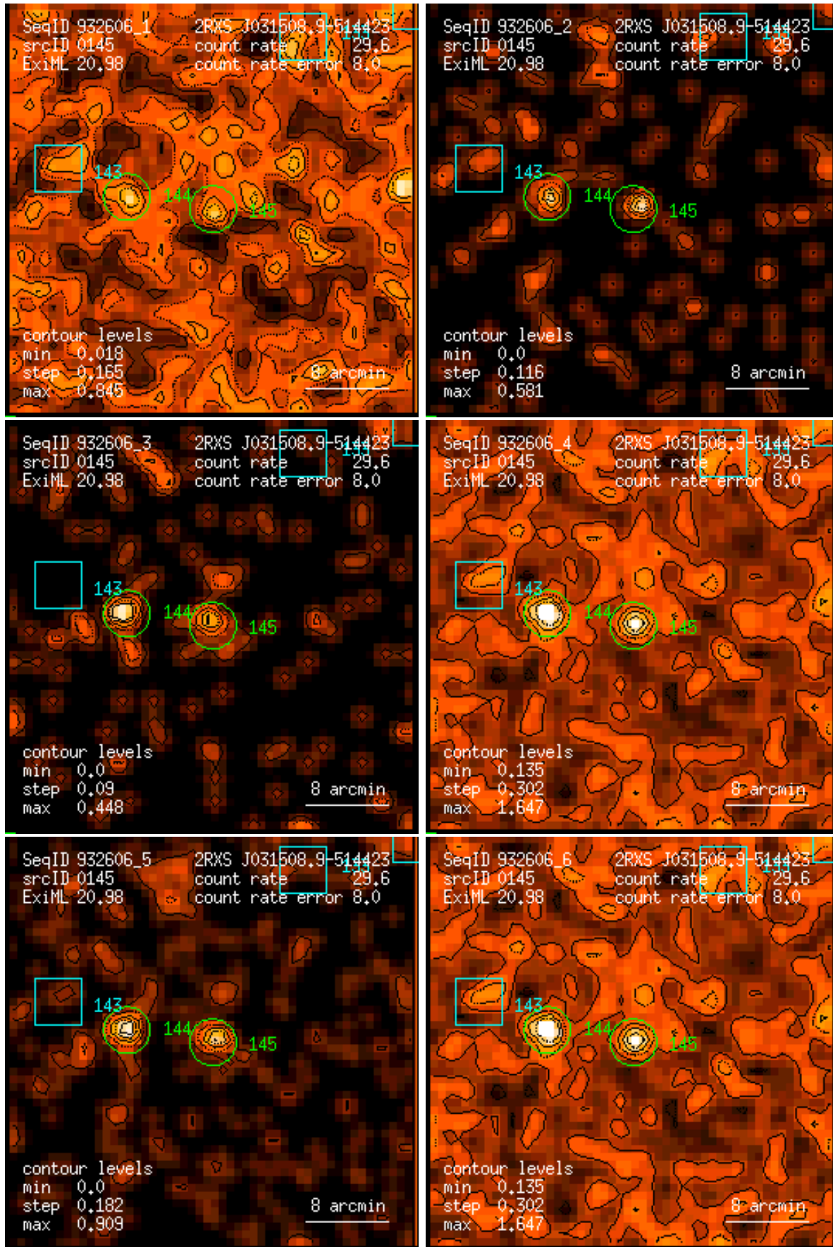
Figure 145: RASS 932606: detection 0145: band rate images, Gaussian filter: (1) PSPC channels 11 – 41, (2) 52 – 90, (3) 91 – 201, (4) 11 – 235, (5) 52 – 201, (6) 11 – 201. Broad band rates in counts/ks. Band rate contour levels in counts/ks/arcmin 2 .
