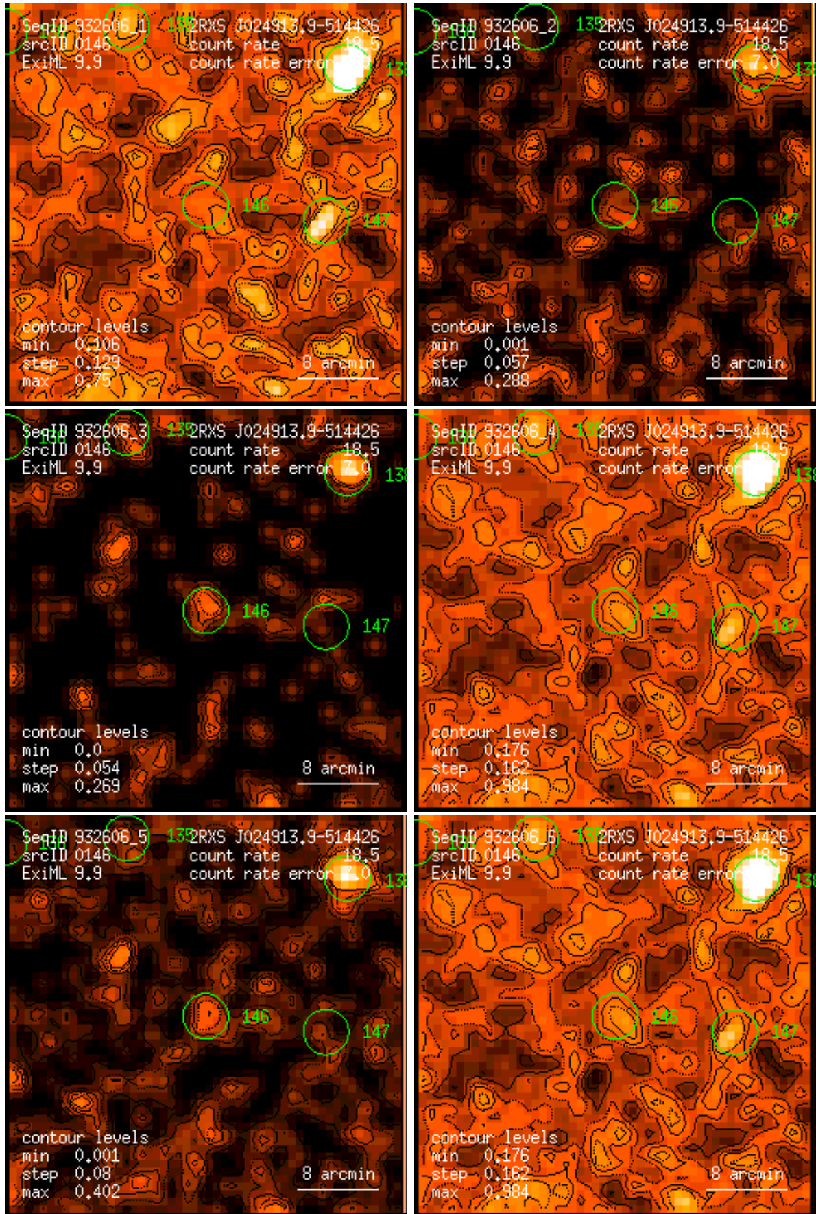
Figure 146: RASS 932606: detection 0146: band rate images, Gaussian filter: (1) PSPC channels 11 – 41, (2) 52 – 90, (3) 91 – 201, (4) 11 – 235, (5) 52 – 201, (6) 11 – 201. Broad band rates in counts/ks. Band rate contour levels in counts/ks/arcmin 2 .
