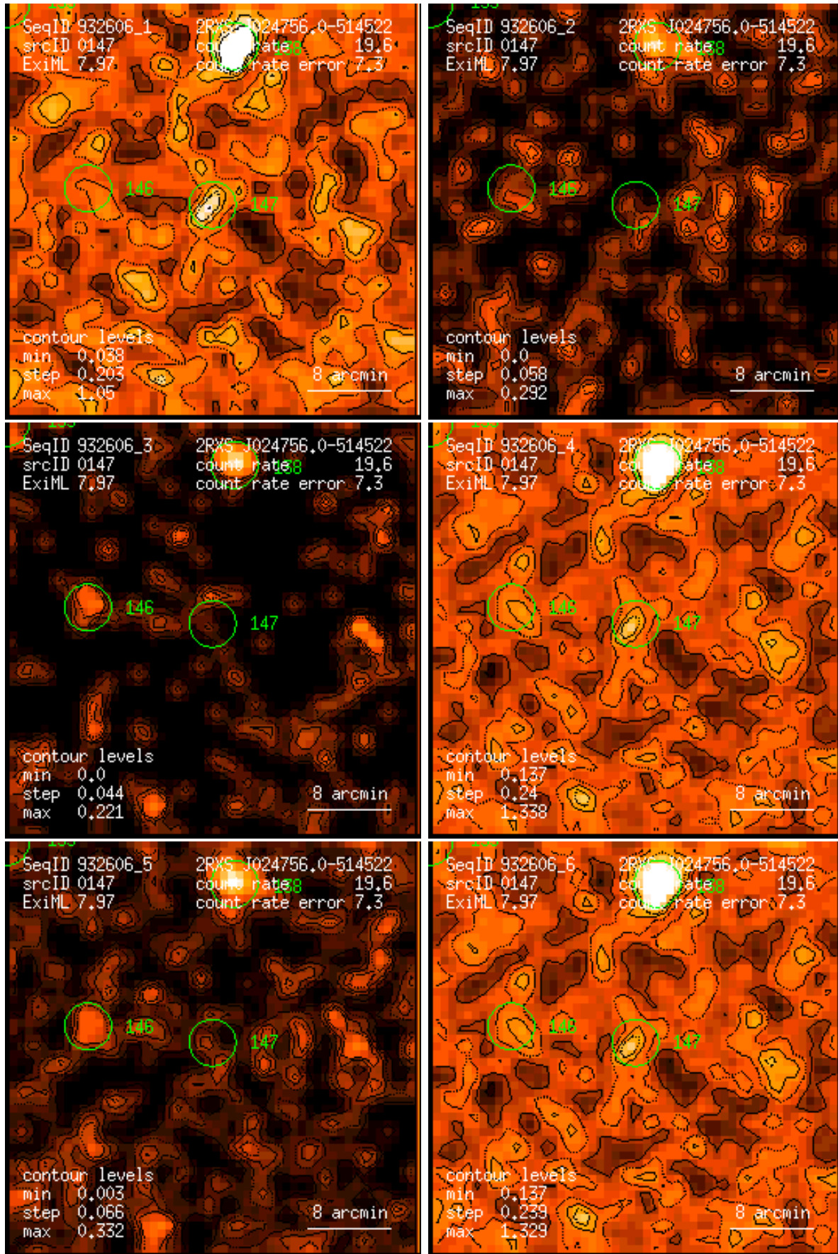
Figure 147: RASS 932606: detection 0147: band rate images, Gaussian filter: (1) PSPC channels 11 – 41, (2) 52 – 90, (3) 91 – 201, (4) 11 – 235, (5) 52 – 201, (6) 11 – 201. Broad band rates in counts/ks. Band rate contour levels in counts/ks/arcmin 2 .
