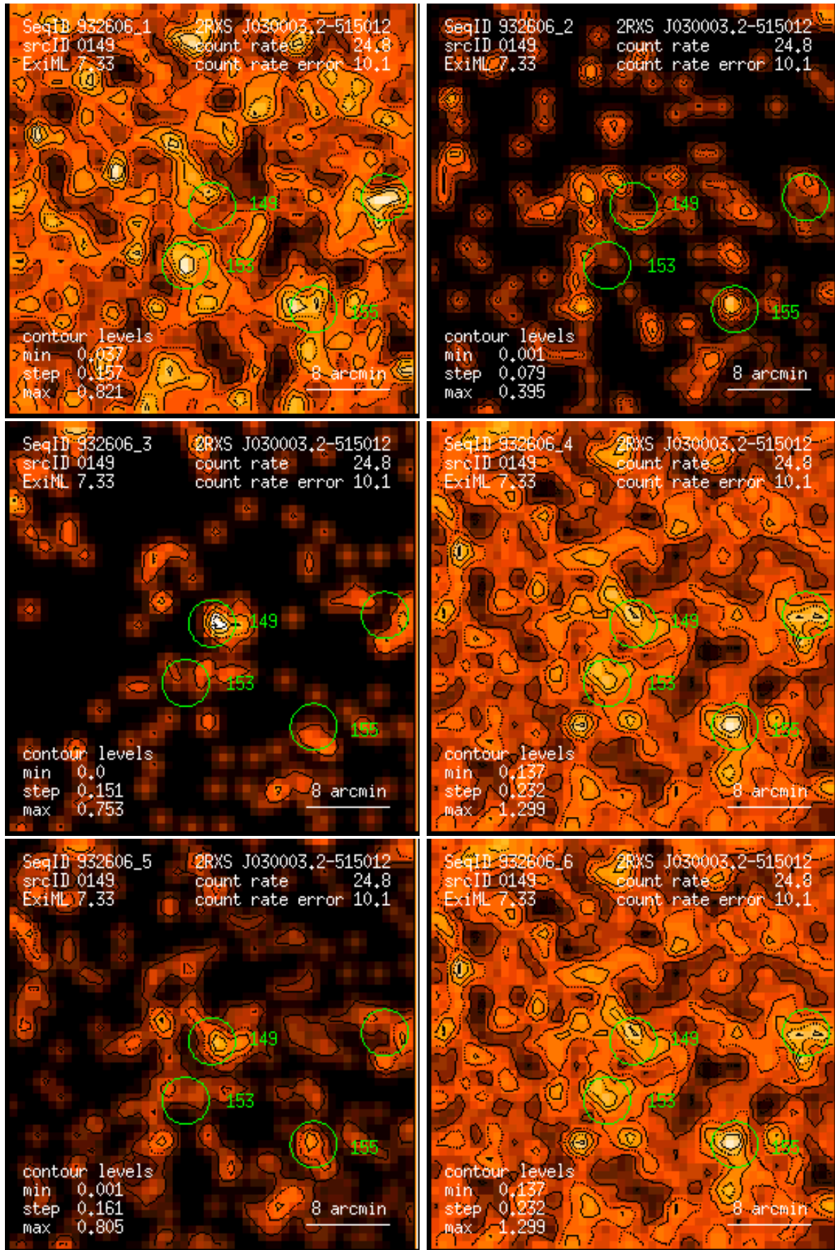
Figure 149: RASS 932606: detection 0149: band rate images, Gaussian filter: (1) PSPC channels 11 – 41, (2) 52 – 90, (3) 91 – 201, (4) 11 – 235, (5) 52 – 201, (6) 11 – 201. Broad band rates in counts/ks. Band rate contour levels in counts/ks/arcmin 2 .
