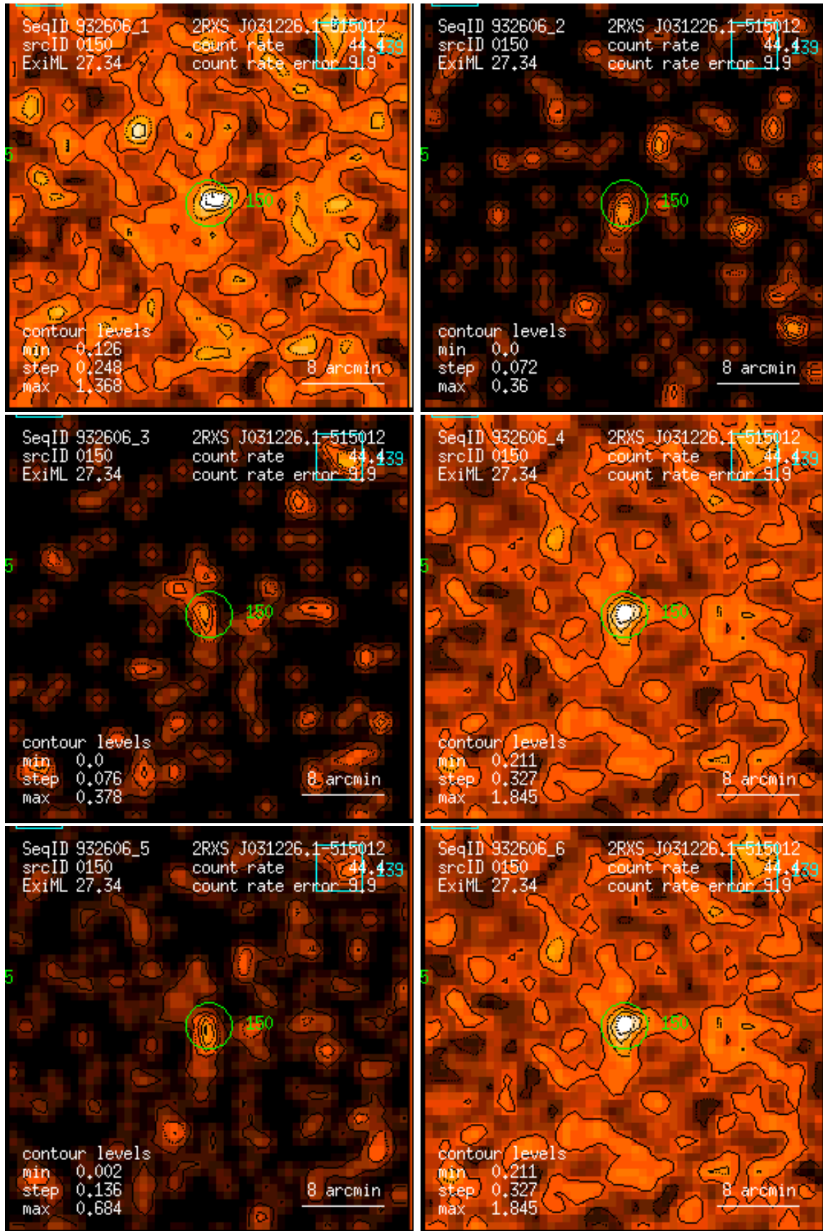
Figure 150: RASS 932606: detection 0150: band rate images, Gaussian filter: (1) PSPC channels 11 – 41, (2) 52 – 90, (3) 91 – 201, (4) 11 – 235, (5) 52 – 201, (6) 11 – 201. Broad band rates in counts/ks. Band rate contour levels in counts/ks/arcmin 2 .
