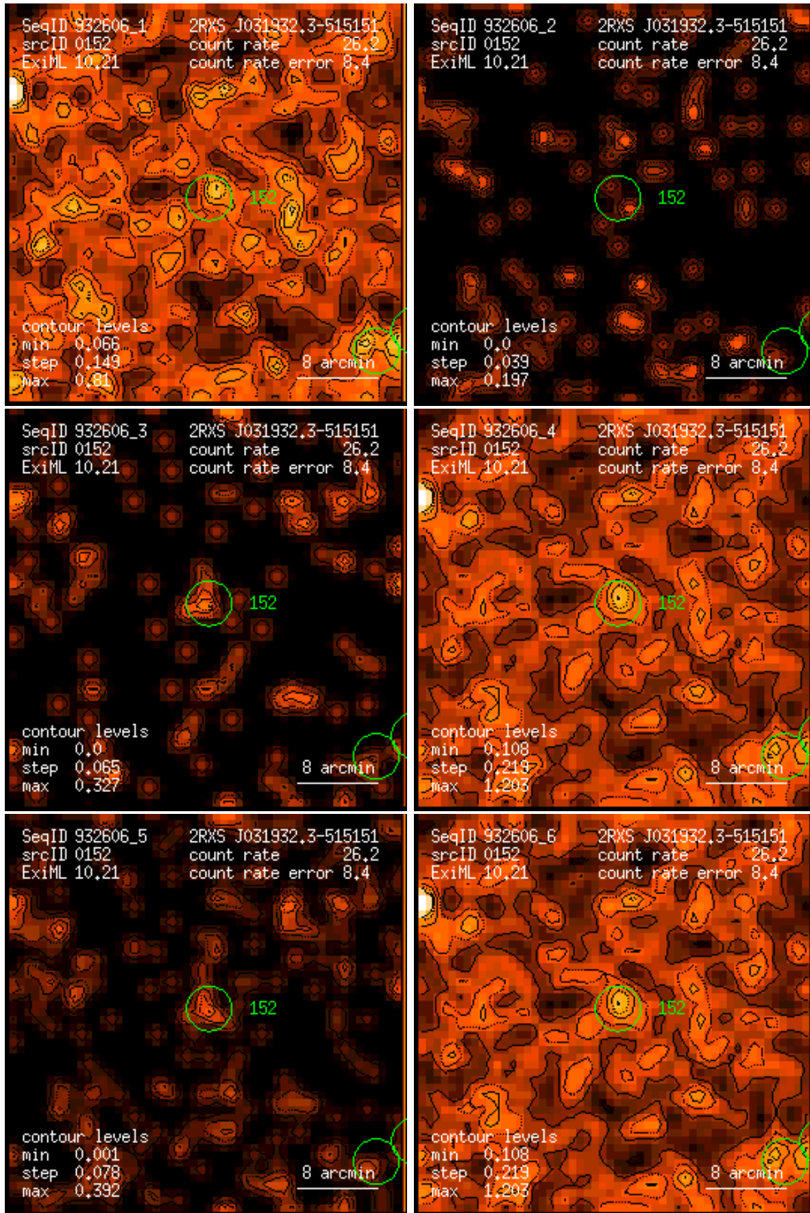
Figure 152: RASS 932606: detection 0152: band rate images, Gaussian filter: (1) PSPC channels 11 – 41, (2) 52 – 90, (3) 91 – 201, (4) 11 – 235, (5) 52 – 201, (6) 11 – 201. Broad band rates in counts/ks. Band rate contour levels in counts/ks/arcmin 2 .
