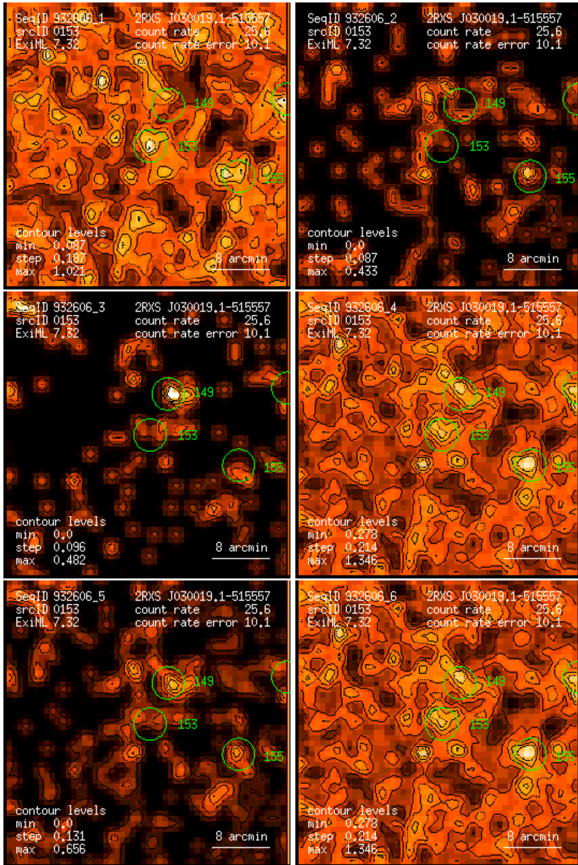
Figure 153: RASS 932606: detection 0153: band rate images, Gaussian filter: (1) PSPC channels 11 – 41, (2) 52 – 90, (3) 91 – 201, (4) 11 – 235, (5) 52 – 201, (6) 11 – 201. Broad band rates in counts/ks. Band rate contour levels in counts/ks/arcmin 2 .
