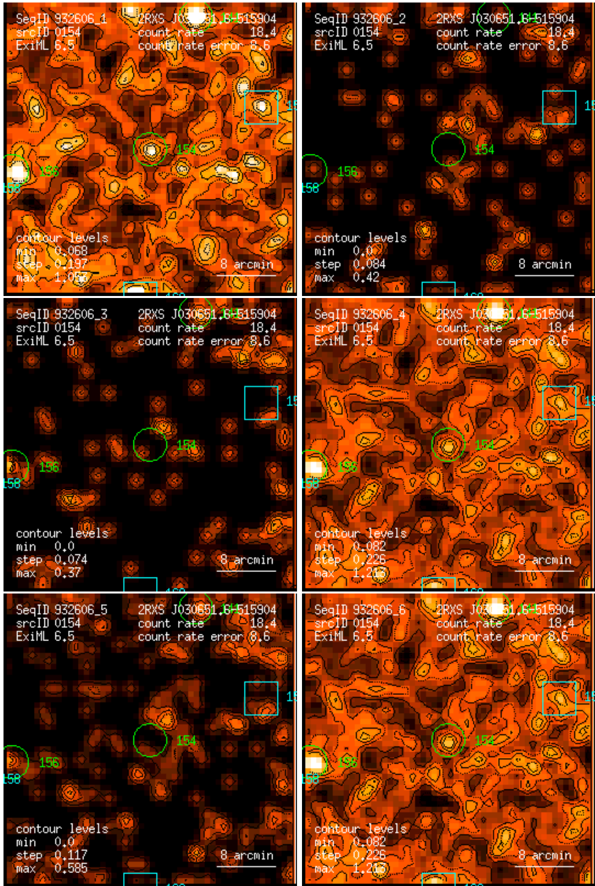
Figure 154: RASS 932606: detection 0154: band rate images, Gaussian filter: (1) PSPC channels 11 – 41, (2) 52 – 90, (3) 91 – 201, (4) 11 – 235, (5) 52 – 201, (6) 11 – 201. Broad band rates in counts/ks. Band rate contour levels in counts/ks/arcmin 2 .
