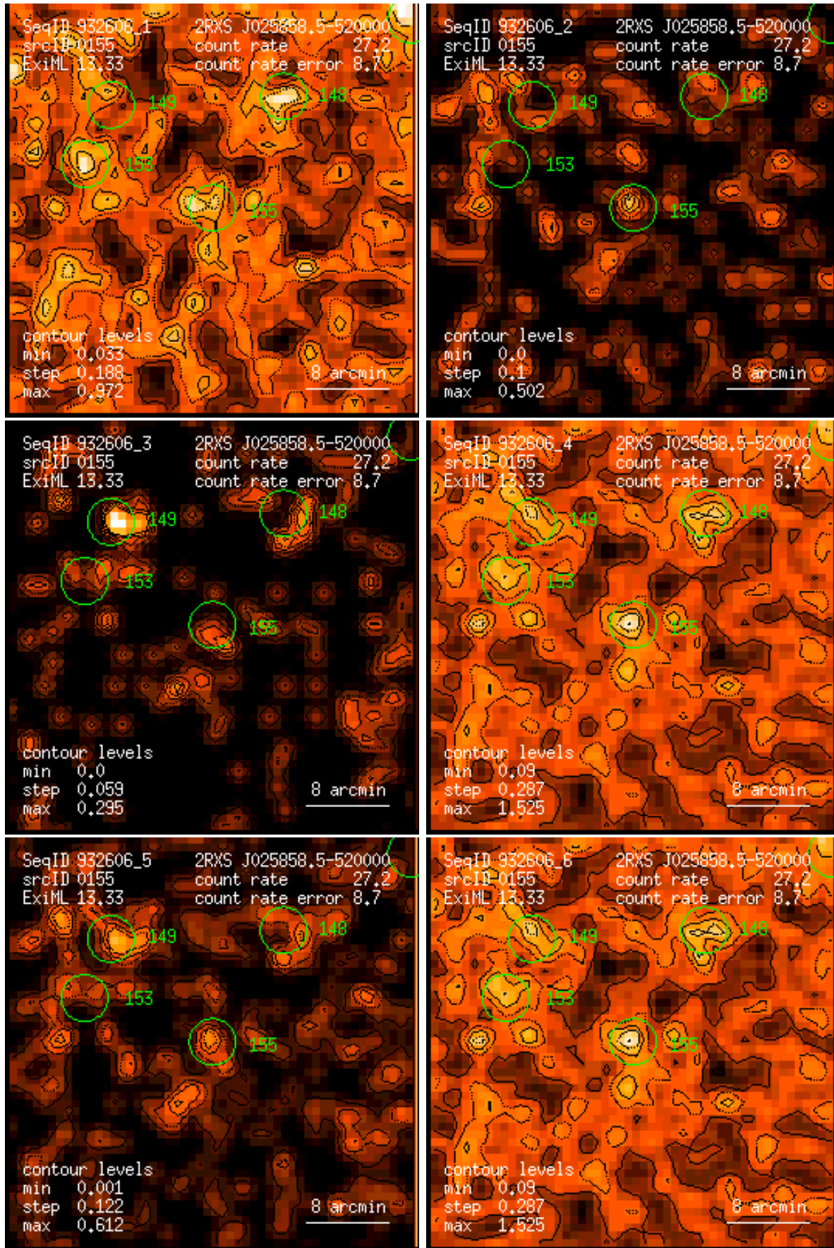
Figure 155: RASS 932606: detection 0155: band rate images, Gaussian filter: (1) PSPC channels 11 – 41, (2) 52 – 90, (3) 91 – 201, (4) 11 – 235, (5) 52 – 201, (6) 11 – 201. Broad band rates in counts/ks. Band rate contour levels in counts/ks/arcmin 2 .
