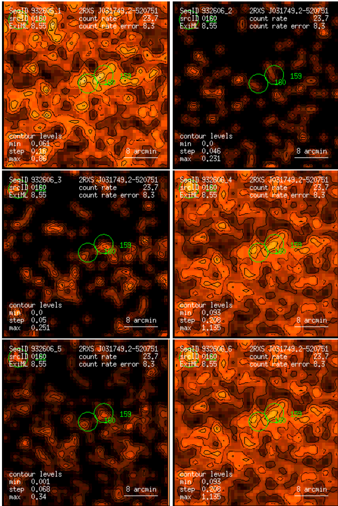
Figure 160: RASS 932606: detection 0160: band rate images, Gaussian filter: (1) PSPC channels 11 – 41, (2) 52 – 90, (3) 91 – 201, (4) 11 – 235, (5) 52 – 201, (6) 11 – 201. Broad band rates in counts/ks. Band rate contour levels in counts/ks/arcmin 2 .
