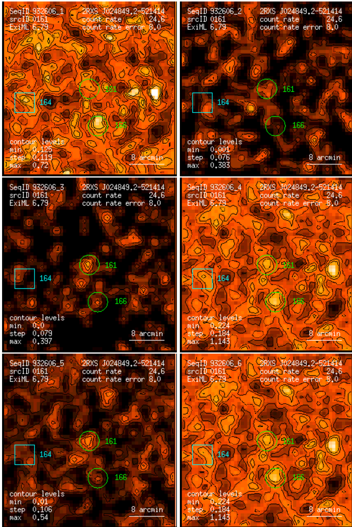
Figure 161: RASS 932606: detection 0161: band rate images, Gaussian filter: (1) PSPC channels 11 – 41, (2) 52 – 90, (3) 91 – 201, (4) 11 – 235, (5) 52 – 201, (6) 11 – 201. Broad band rates in counts/ks. Band rate contour levels in counts/ks/arcmin 2 .
