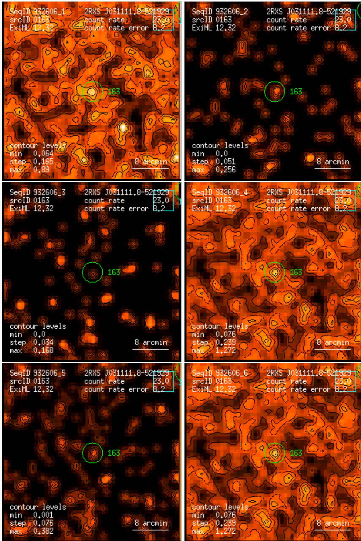
Figure 163: RASS 932606: detection 0163: band rate images, Gaussian filter: (1) PSPC channels 11 – 41, (2) 52 – 90, (3) 91 – 201, (4) 11 – 235, (5) 52 – 201, (6) 11 – 201. Broad band rates in counts/ks. Band rate contour levels in counts/ks/arcmin 2 .
